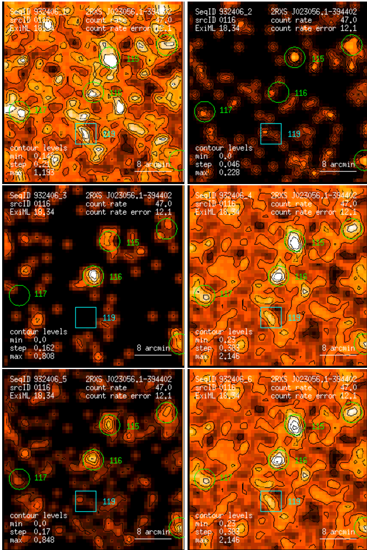
Figure 116: RASS 932406: detection 0116: band rate images, Gaussian filter: (1) PSPC channels 11 – 41, (2) 52 – 90, (3) 91 – 201, (4) 11 – 235, (5) 52 – 201, (6) 11 – 201. Broad band rates in counts/ks. Band rate contour levels in counts/ks/arcmin 2 .
