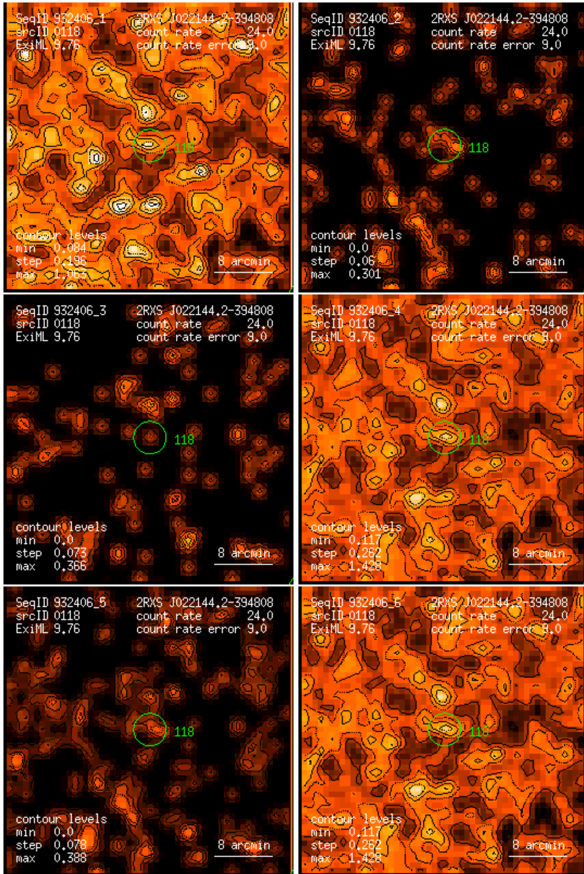
Figure 118: RASS 932406: detection 0118: band rate images, Gaussian filter: (1) PSPC channels 11 – 41, (2) 52 – 90, (3) 91 – 201, (4) 11 – 235, (5) 52 – 201, (6) 11 – 201. Broad band rates in counts/ks. Band rate contour levels in counts/ks/arcmin 2 .
