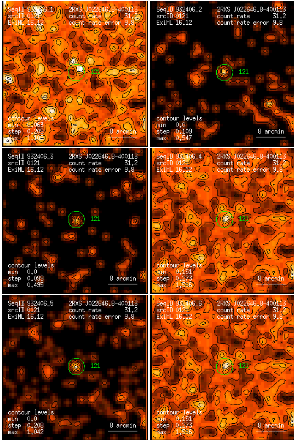
Figure 121: RASS 932406: detection 0121: band rate images, Gaussian filter: (1) PSPC channels 11 – 41, (2) 52 – 90, (3) 91 – 201, (4) 11 – 235, (5) 52 – 201, (6) 11 – 201. Broad band rates in counts/ks. Band rate contour levels in counts/ks/arcmin 2 .
