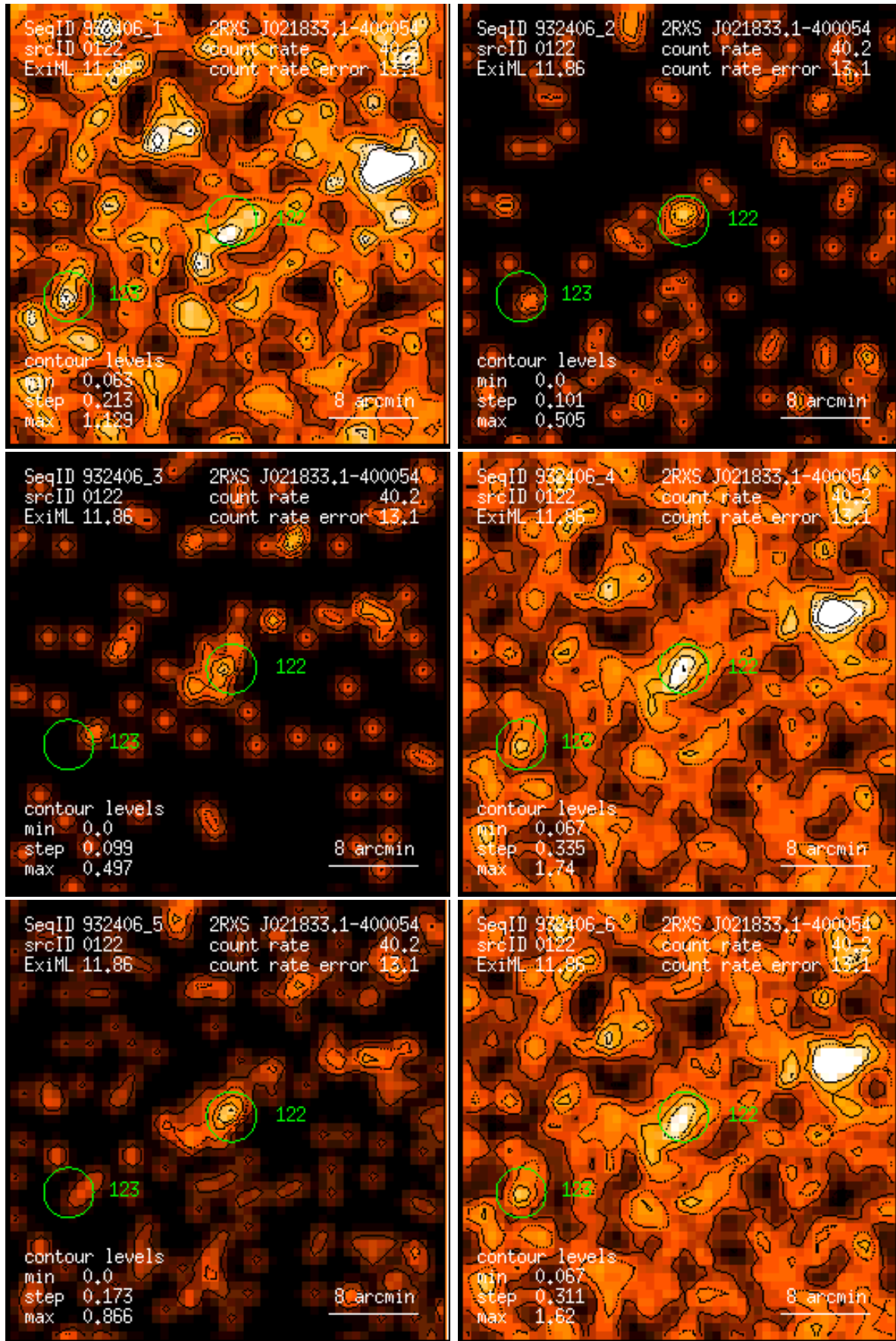
Figure 122: RASS 932406: detection 0122: band rate images, Gaussian filter: (1) PSPC channels 11 – 41, (2) 52 – 90, (3) 91 – 201, (4) 11 – 235, (5) 52 – 201, (6) 11 – 201. Broad band rates in counts/ks. Band rate contour levels in counts/ks/arcmin 2 .
