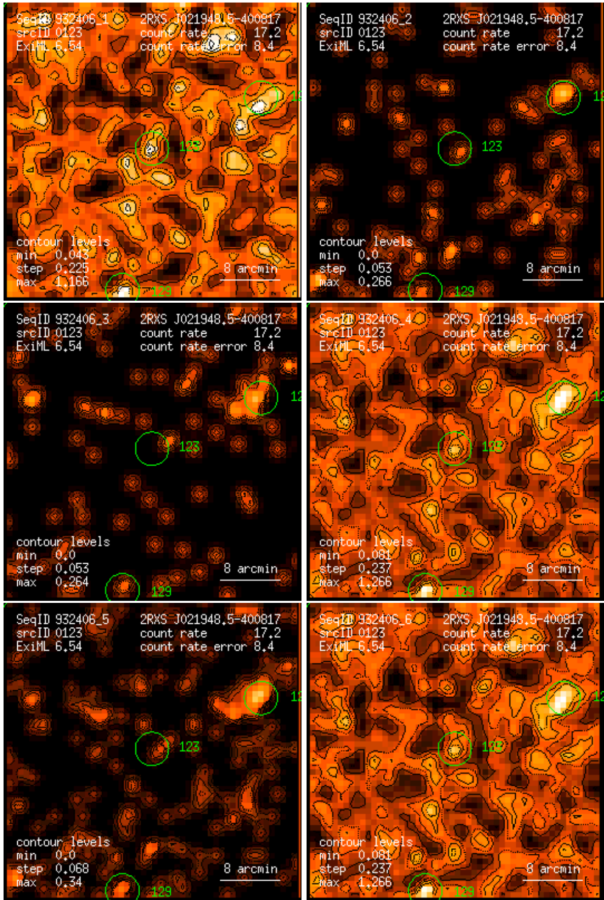
Figure 123: RASS 932406: detection 0123: band rate images, Gaussian filter: (1) PSPC channels 11 – 41, (2) 52 – 90, (3) 91 – 201, (4) 11 – 235, (5) 52 – 201, (6) 11 – 201. Broad band rates in counts/ks. Band rate contour levels in counts/ks/arcmin 2 .
