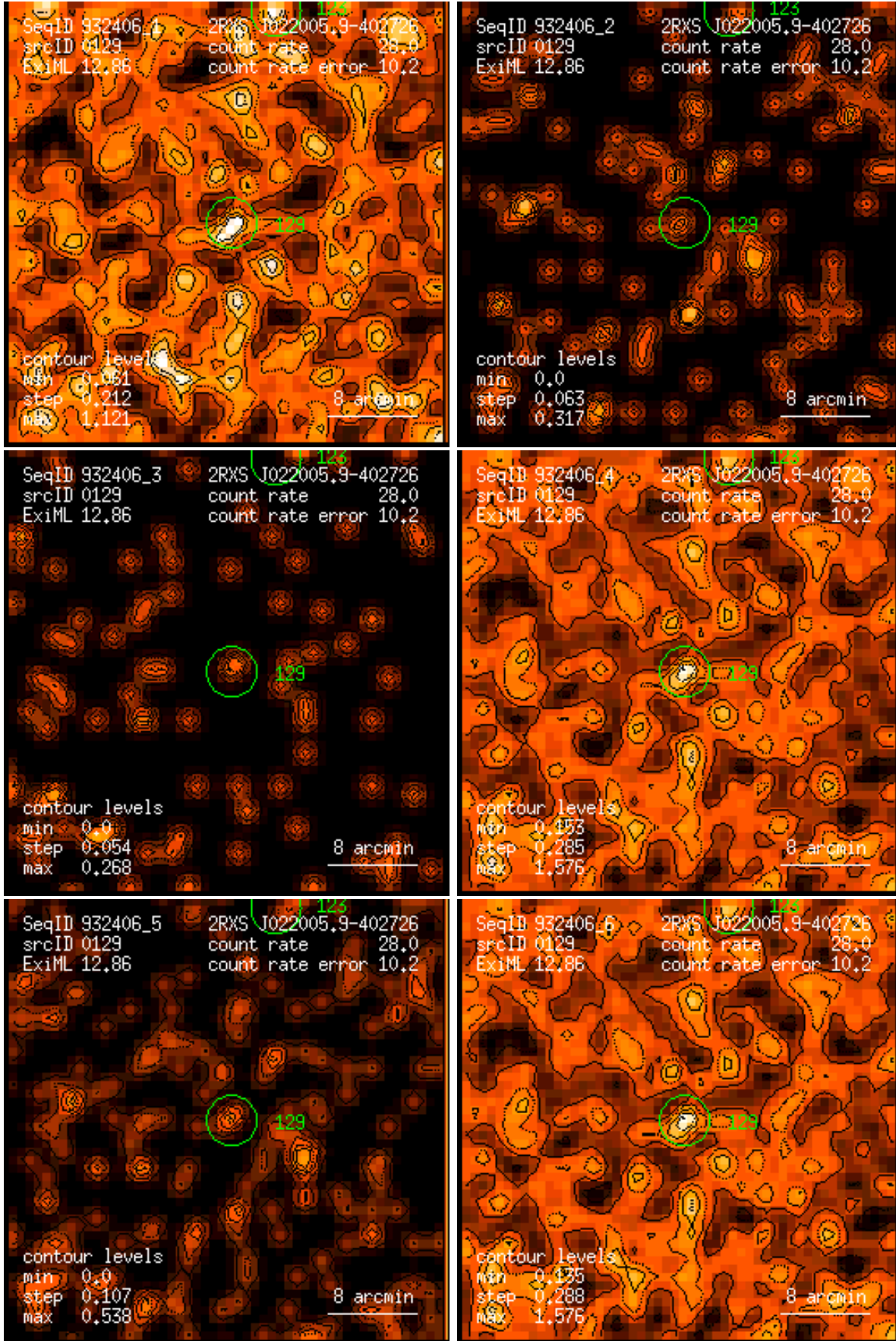
Figure 129: RASS 932406: detection 0129: band rate images, Gaussian filter: (1) PSPC channels 11 – 41, (2) 52 – 90, (3) 91 – 201, (4) 11 – 235, (5) 52 – 201, (6) 11 – 201. Broad band rates in counts/ks. Band rate contour levels in counts/ks/arcmin 2 .
