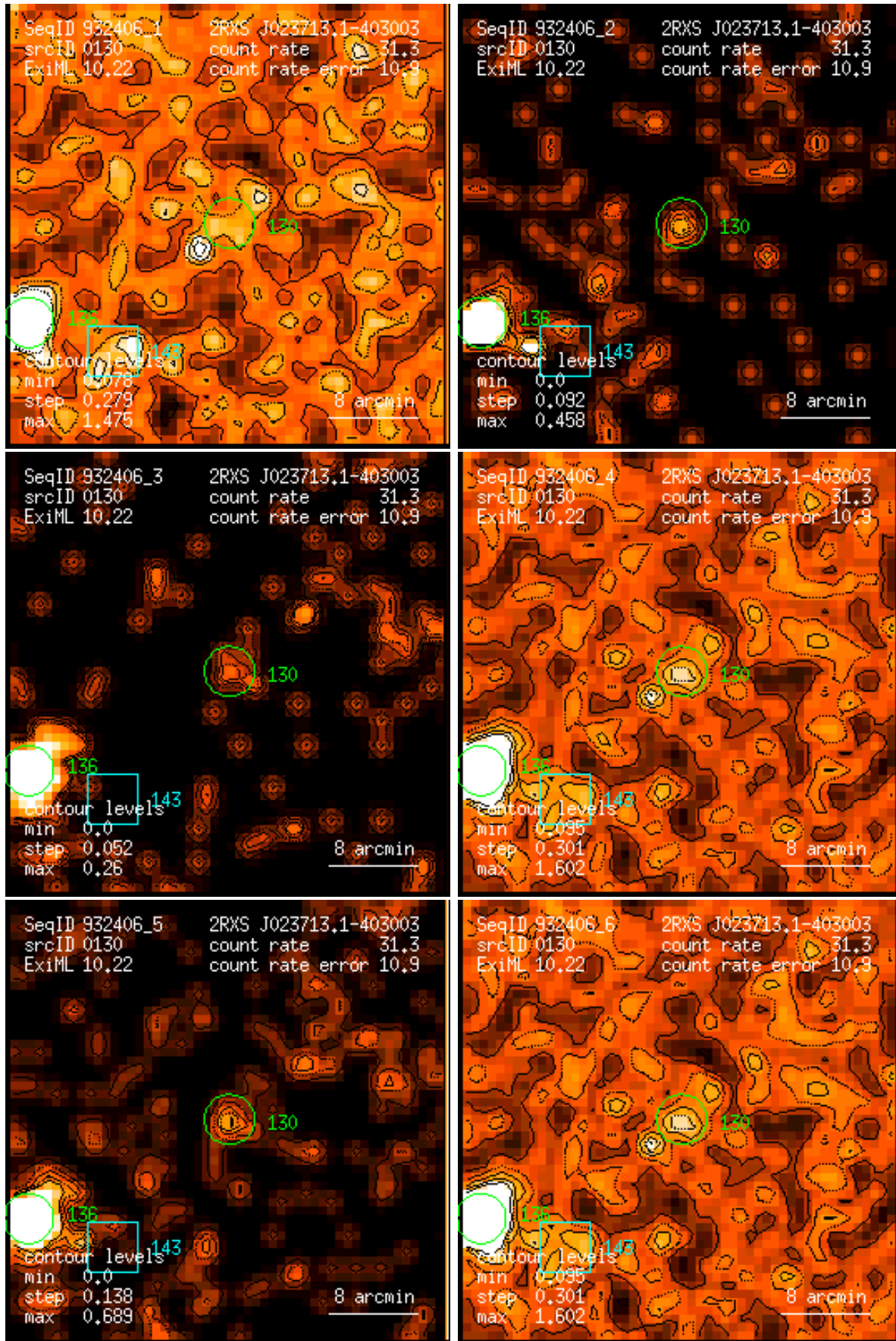
Figure 130: RASS 932406: detection 0130: band rate images, Gaussian filter: (1) PSPC channels 11 – 41, (2) 52 – 90, (3) 91 – 201, (4) 11 – 235, (5) 52 – 201, (6) 11 – 201. Broad band rates in counts/ks. Band rate contour levels in counts/ks/arcmin 2 .
