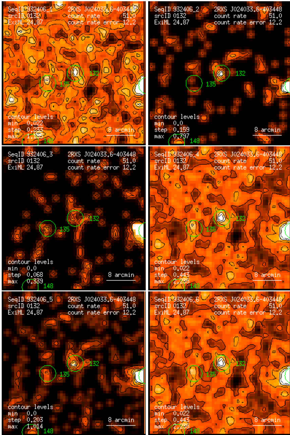
Figure 132: RASS 932406: detection 0132: band rate images, Gaussian filter: (1) PSPC channels 11 – 41, (2) 52 – 90, (3) 91 – 201, (4) 11 – 235, (5) 52 – 201, (6) 11 – 201. Broad band rates in counts/ks. Band rate contour levels in counts/ks/arcmin 2 .
