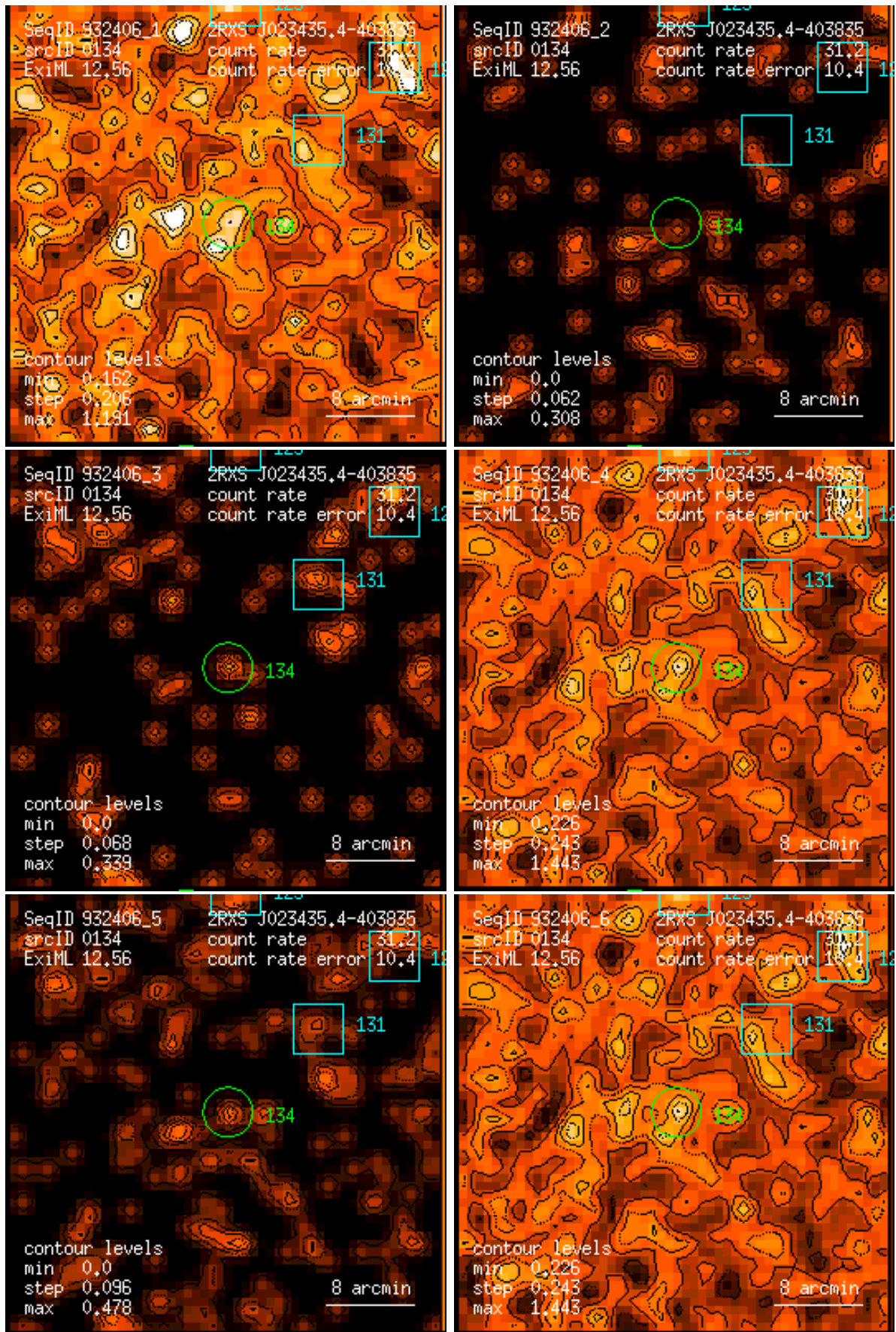
Figure 134: RASS 932406: detection 0134: band rate images, Gaussian filter: (1) PSPC channels 11 – 41, (2) 52 – 90, (3) 91 – 201, (4) 11 – 235, (5) 52 – 201, (6) 11 – 201. Broad band rates in counts/ks. Band rate contour levels in counts/ks/arcmin 2 .
