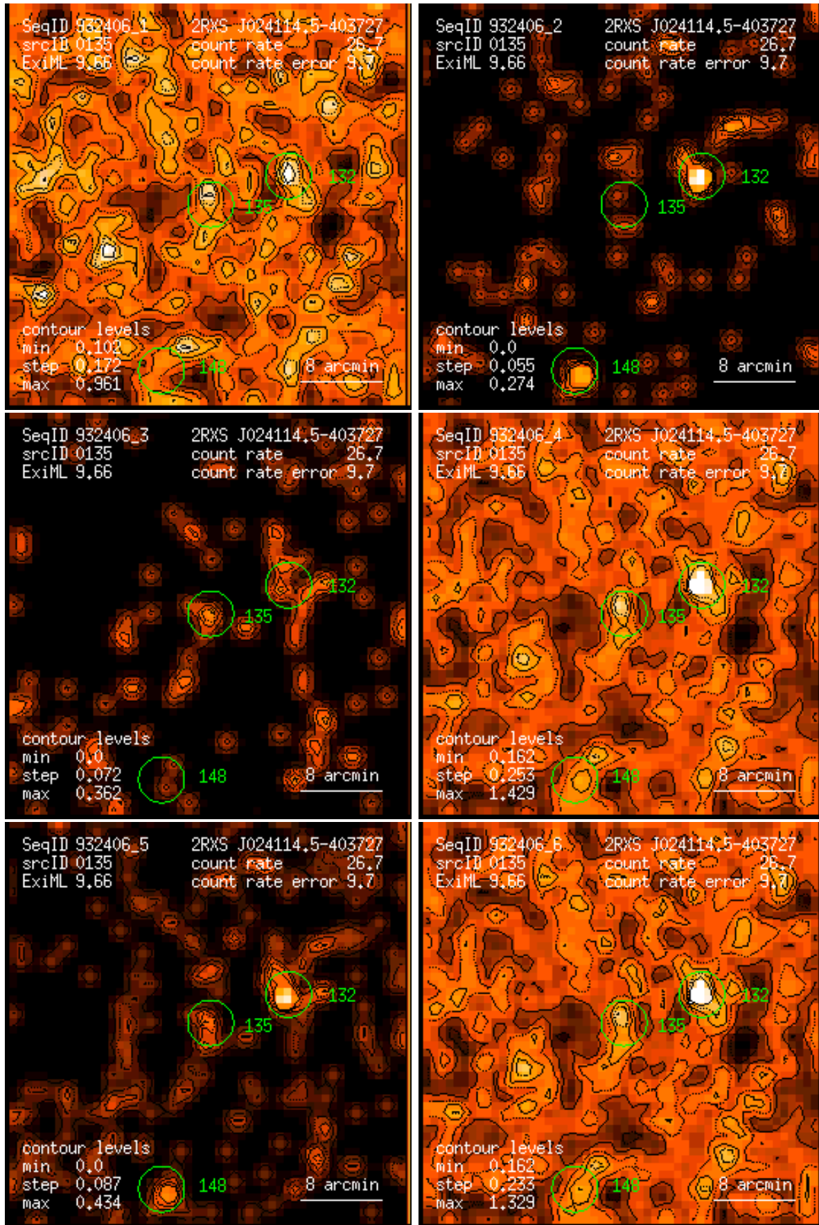
Figure 135: RASS 932406: detection 0135: band rate images, Gaussian filter: (1) PSPC channels 11 – 41, (2) 52 – 90, (3) 91 – 201, (4) 11 – 235, (5) 52 – 201, (6) 11 – 201. Broad band rates in counts/ks. Band rate contour levels in counts/ks/arcmin 2 .
