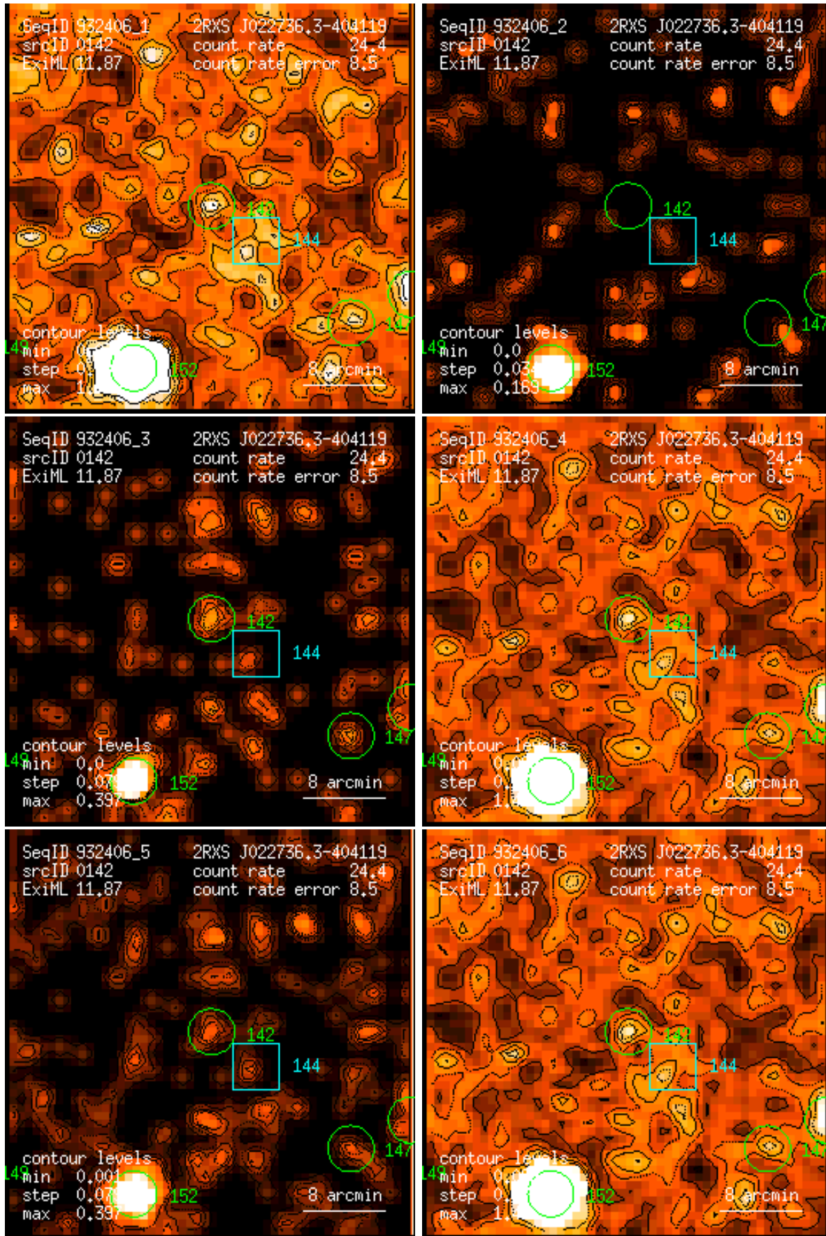
Figure 142: RASS 932406: detection 0142: band rate images, Gaussian filter: (1) PSPC channels 11 – 41, (2) 52 – 90, (3) 91 – 201, (4) 11 – 235, (5) 52 – 201, (6) 11 – 201. Broad band rates in counts/ks. Band rate contour levels in counts/ks/arcmin 2 .
