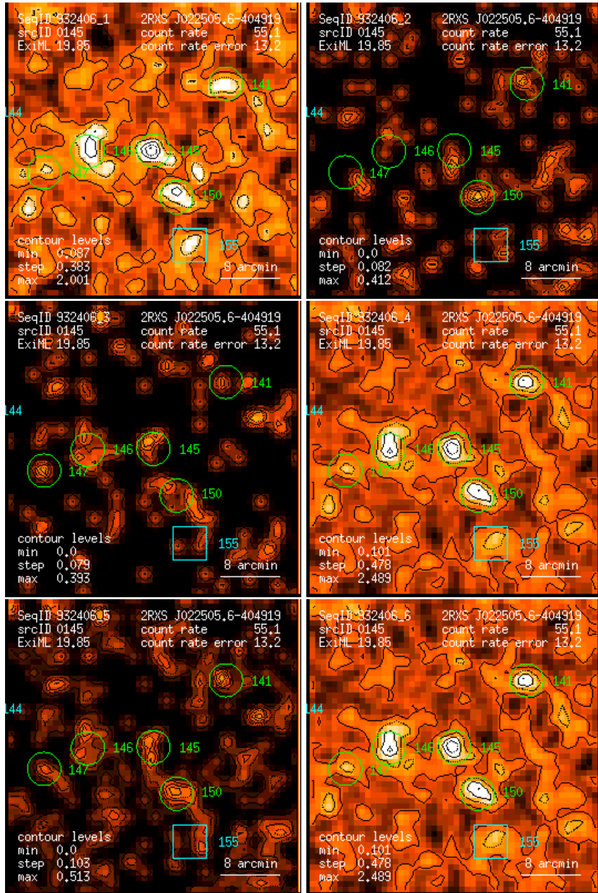
Figure 145: RASS 932406: detection 0145: band rate images, Gaussian filter: (1) PSPC channels 11 – 41, (2) 52 – 90, (3) 91 – 201, (4) 11 – 235, (5) 52 – 201, (6) 11 – 201. Broad band rates in counts/ks. Band rate contour levels in counts/ks/arcmin 2 .
