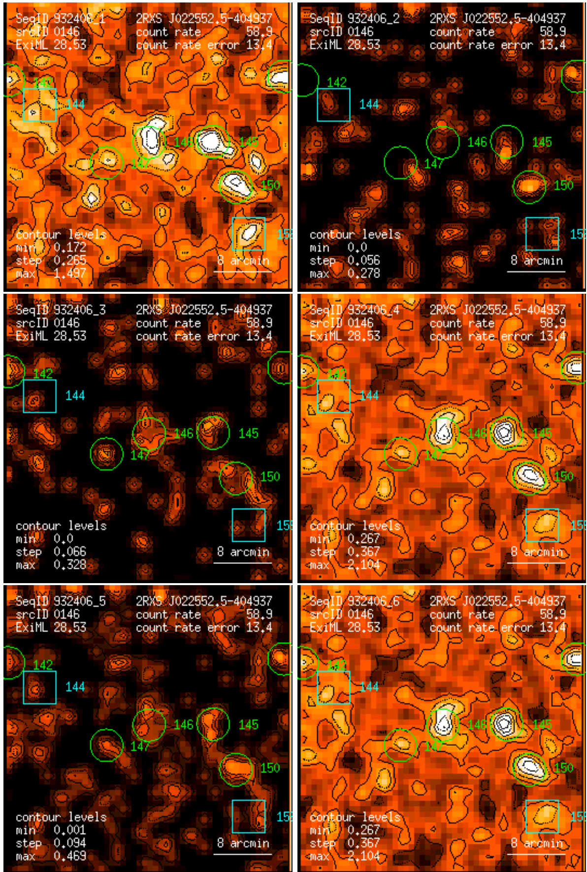
Figure 146: RASS 932406: detection 0146: band rate images, Gaussian filter: (1) PSPC channels 11 – 41, (2) 52 – 90, (3) 91 – 201, (4) 11 – 235, (5) 52 – 201, (6) 11 – 201. Broad band rates in counts/ks. Band rate contour levels in counts/ks/arcmin 2 .
