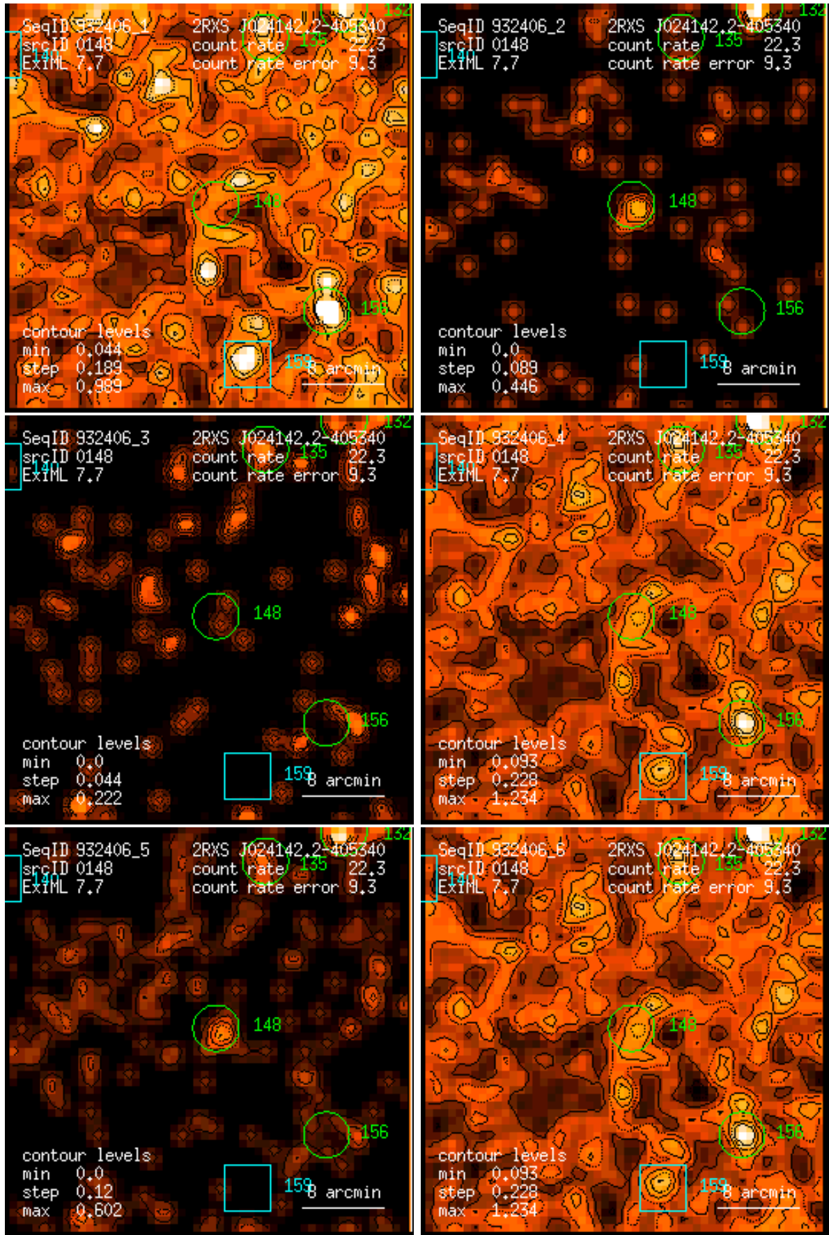
Figure 148: RASS 932406: detection 0148: band rate images, Gaussian filter: (1) PSPC channels 11 – 41, (2) 52 – 90, (3) 91 – 201, (4) 11 – 235, (5) 52 – 201, (6) 11 – 201. Broad band rates in counts/ks. Band rate contour levels in counts/ks/arcmin 2 .
