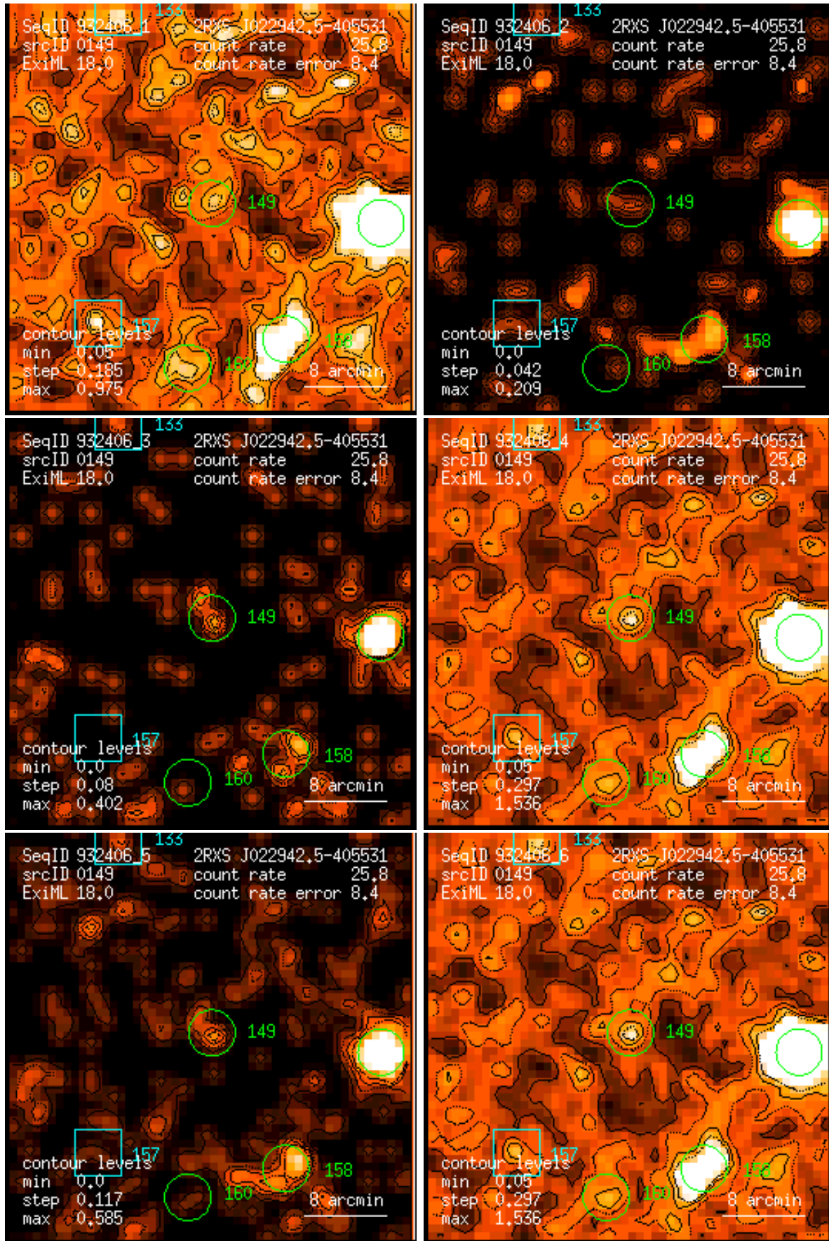
Figure 149: RASS 932406: detection 0149: band rate images, Gaussian filter: (1) PSPC channels 11 – 41, (2) 52 – 90, (3) 91 – 201, (4) 11 – 235, (5) 52 – 201, (6) 11 – 201. Broad band rates in counts/ks. Band rate contour levels in counts/ks/arcmin 2 .
