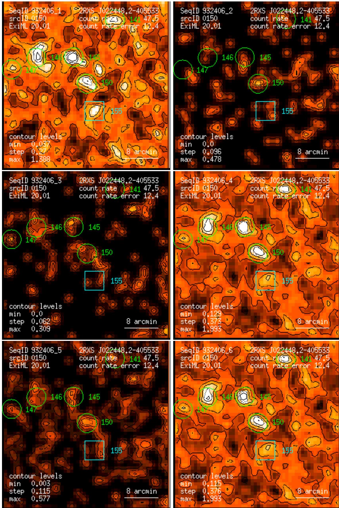
Figure 150: RASS 932406: detection 0150: band rate images, Gaussian filter: (1) PSPC channels 11 – 41, (2) 52 – 90, (3) 91 – 201, (4) 11 – 235, (5) 52 – 201, (6) 11 – 201. Broad band rates in counts/ks. Band rate contour levels in counts/ks/arcmin 2 .
