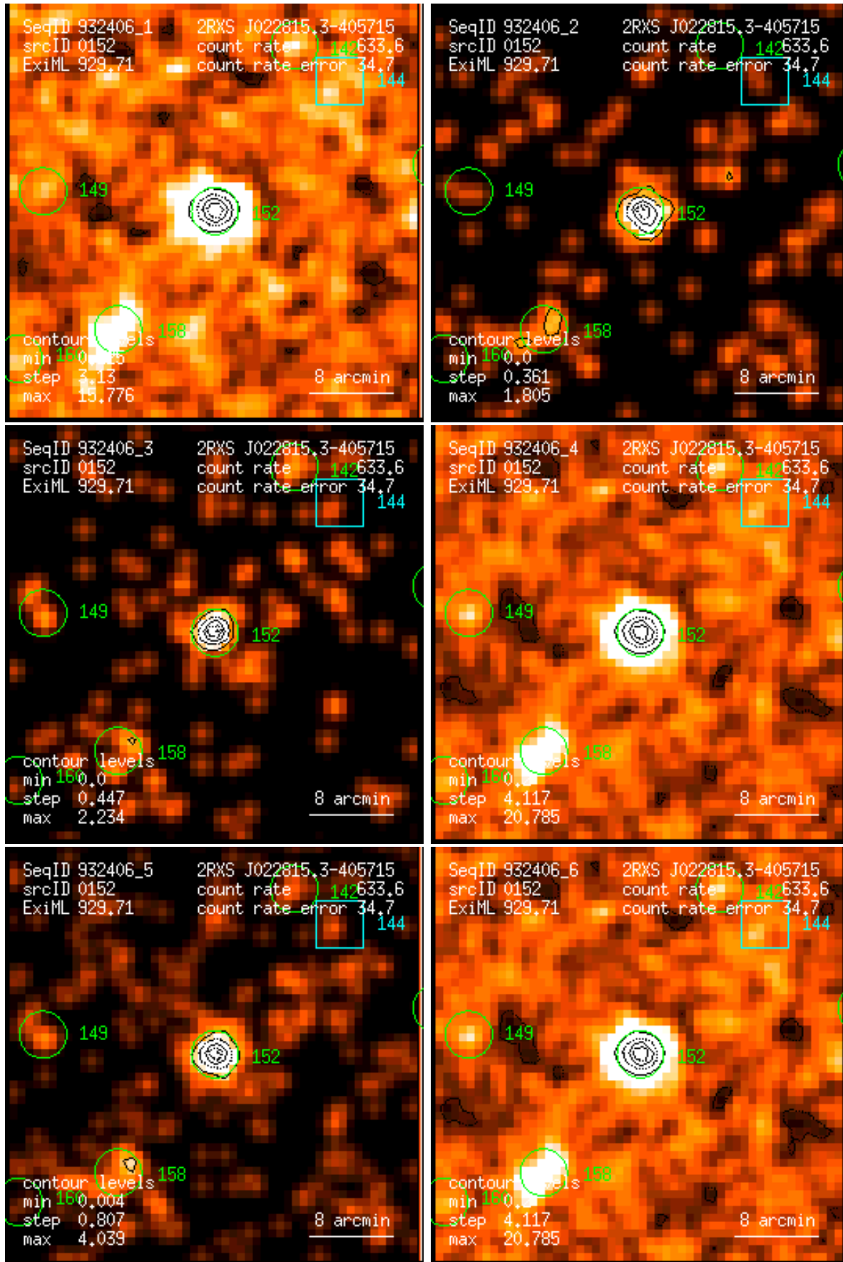
Figure 152: RASS 932406: detection 0152: band rate images, Gaussian filter: (1) PSPC channels 11 – 41, (2) 52 – 90, (3) 91 – 201, (4) 11 – 235, (5) 52 – 201, (6) 11 – 201. Broad band rates in counts/ks. Band rate contour levels in counts/ks/arcmin 2 .
