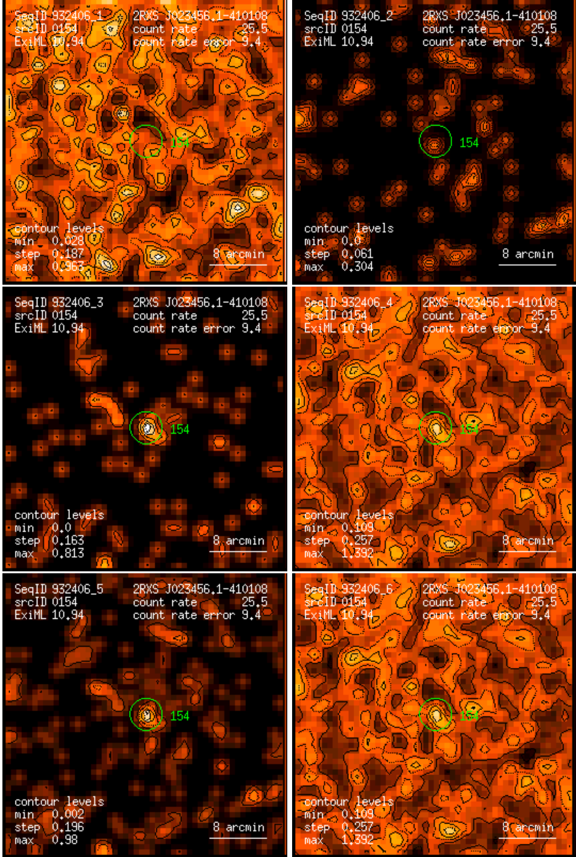
Figure 154: RASS 932406: detection 0154: band rate images, Gaussian filter: (1) PSPC channels 11 – 41, (2) 52 – 90, (3) 91 – 201, (4) 11 – 235, (5) 52 – 201, (6) 11 – 201. Broad band rates in counts/ks. Band rate contour levels in counts/ks/arcmin 2 .
