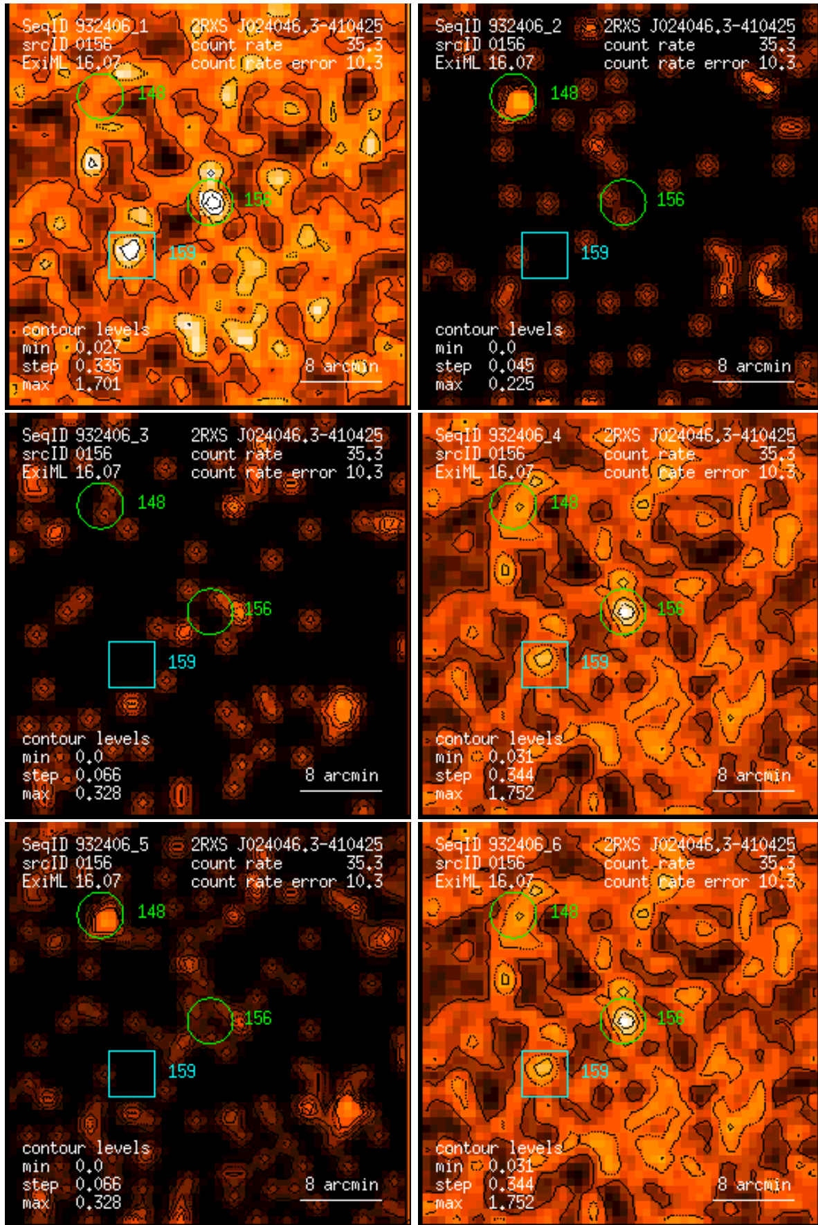
Figure 156: RASS 932406: detection 0156: band rate images, Gaussian filter: (1) PSPC channels 11 – 41, (2) 52 – 90, (3) 91 – 201, (4) 11 – 235, (5) 52 – 201, (6) 11 – 201. Broad band rates in counts/ks. Band rate contour levels in counts/ks/arcmin 2 .
