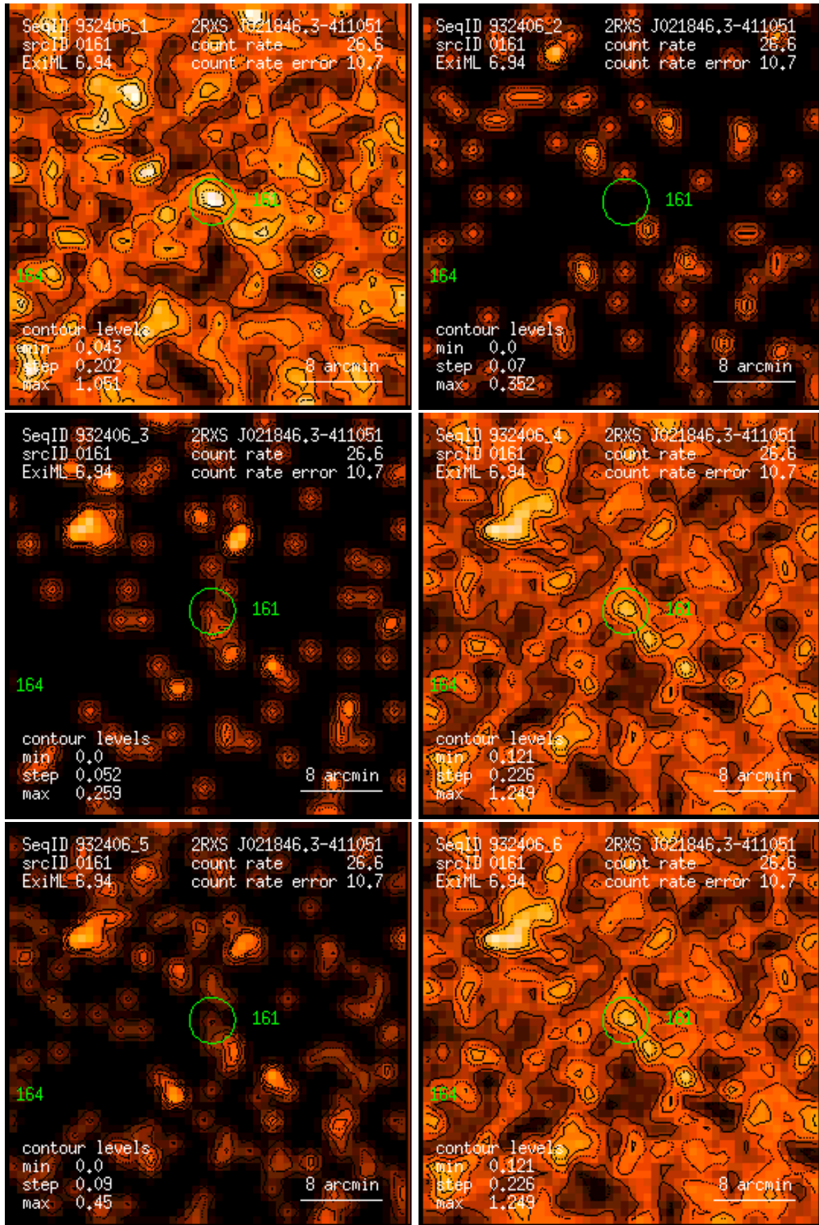
Figure 161: RASS 932406: detection 0161: band rate images, Gaussian filter: (1) PSPC channels 11 – 41, (2) 52 – 90, (3) 91 – 201, (4) 11 – 235, (5) 52 – 201, (6) 11 – 201. Broad band rates in counts/ks. Band rate contour levels in counts/ks/arcmin 2 .
