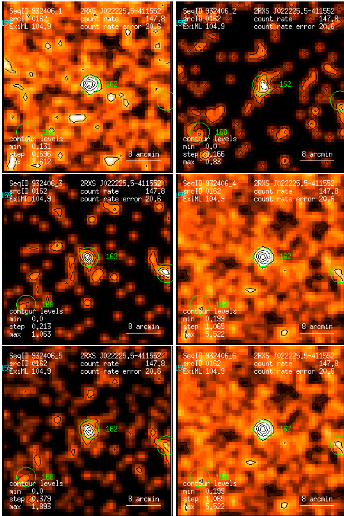
Figure 162: RASS 932406: detection 0162: band rate images, Gaussian filter: (1) PSPC channels 11 – 41, (2) 52 – 90, (3) 91 – 201, (4) 11 – 235, (5) 52 – 201, (6) 11 – 201. Broad band rates in counts/ks. Band rate contour levels in counts/ks/arcmin 2 .
