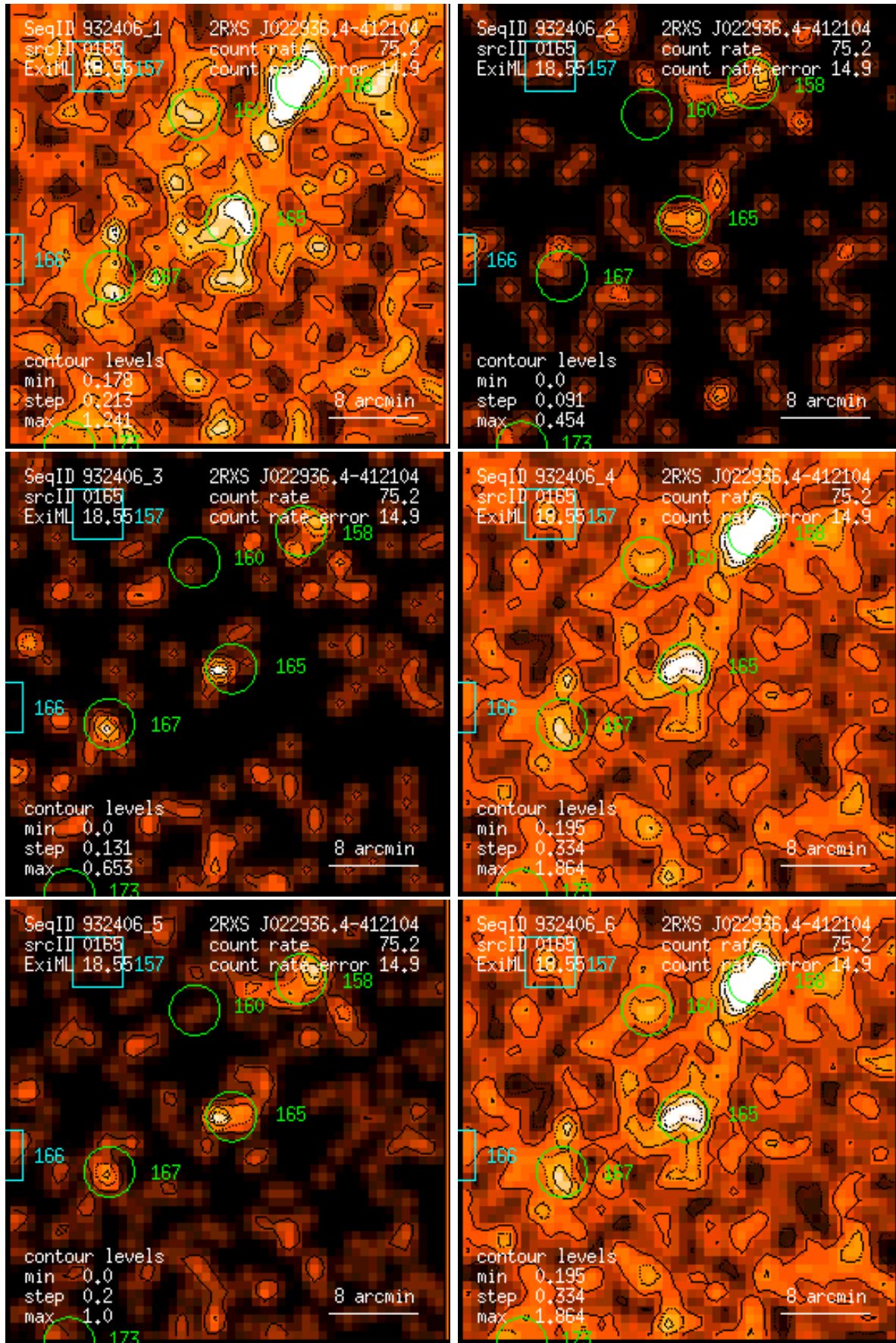
Figure 165: RASS 932406: detection 0165: band rate images, Gaussian filter: (1) PSPC channels 11 – 41, (2) 52 – 90, (3) 91 – 201, (4) 11 – 235, (5) 52 – 201, (6) 11 – 201. Broad band rates in counts/ks. Band rate contour levels in counts/ks/arcmin 2 .
