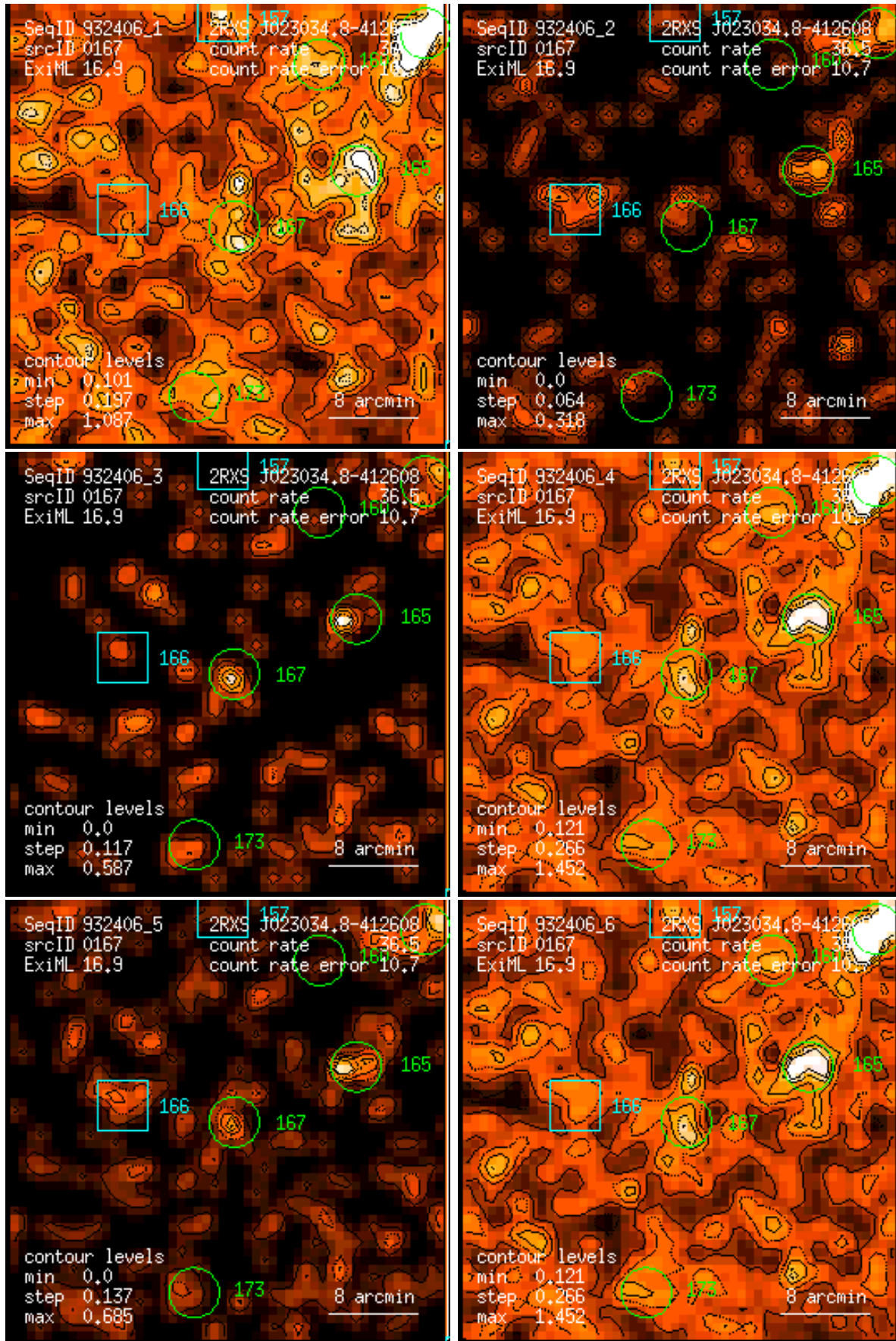
Figure 167: RASS 932406: detection 0167: band rate images, Gaussian filter: (1) PSPC channels 11 – 41, (2) 52 – 90, (3) 91 – 201, (4) 11 – 235, (5) 52 – 201, (6) 11 – 201. Broad band rates in counts/ks. Band rate contour levels in counts/ks/arcmin 2 .
