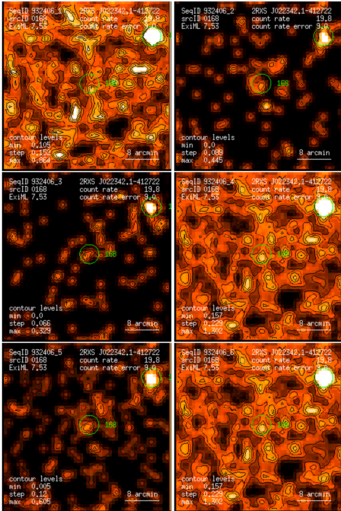
Figure 168: RASS 932406: detection 0168: band rate images, Gaussian filter: (1) PSPC channels 11 – 41, (2) 52 – 90, (3) 91 – 201, (4) 11 – 235, (5) 52 – 201, (6) 11 – 201. Broad band rates in counts/ks. Band rate contour levels in counts/ks/arcmin 2 .
