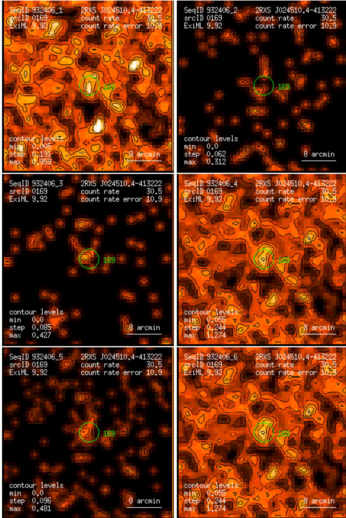
Figure 169: RASS 932406: detection 0169: band rate images, Gaussian filter: (1) PSPC channels 11 – 41, (2) 52 – 90, (3) 91 – 201, (4) 11 – 235, (5) 52 – 201, (6) 11 – 201. Broad band rates in counts/ks. Band rate contour levels in counts/ks/arcmin 2 .
