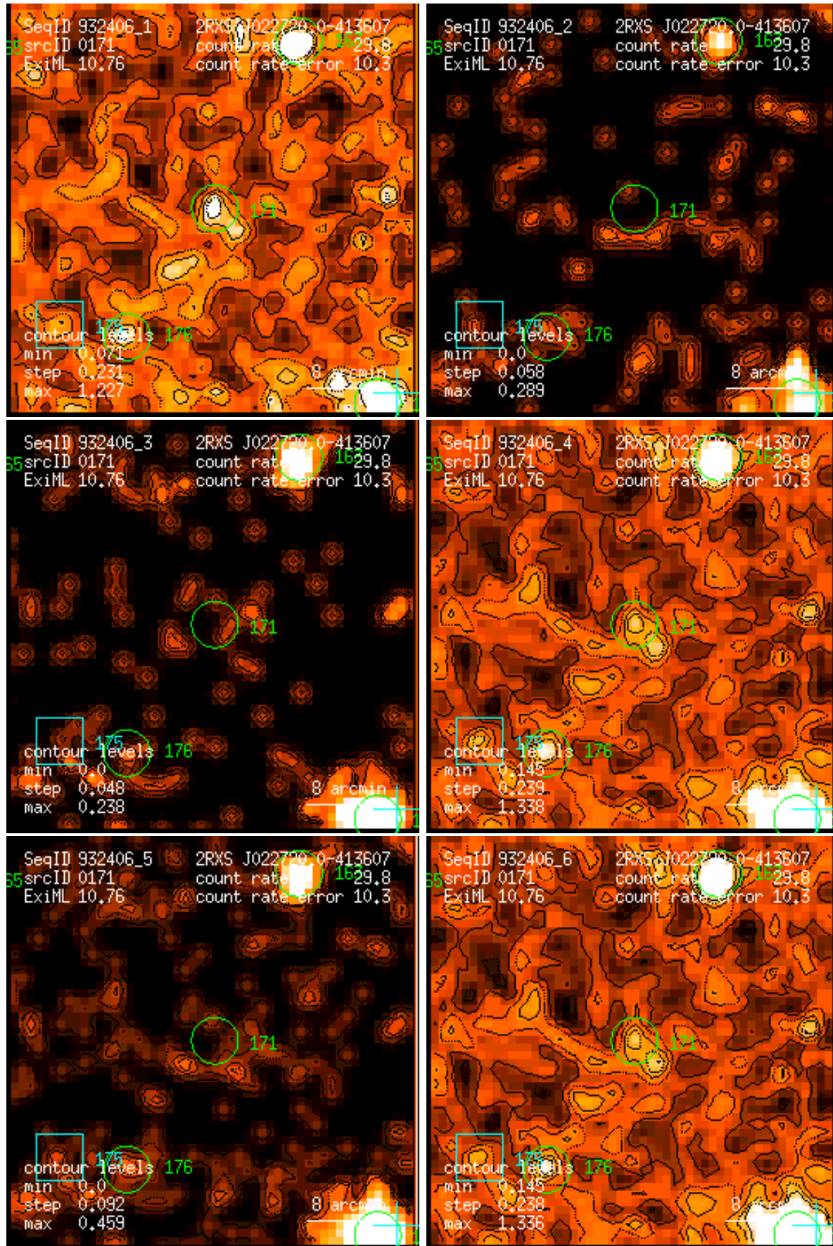
Figure 171: RASS 932406: detection 0171: band rate images, Gaussian filter: (1) PSPC channels 11 – 41, (2) 52 – 90, (3) 91 – 201, (4) 11 – 235, (5) 52 – 201, (6) 11 – 201. Broad band rates in counts/ks. Band rate contour levels in counts/ks/arcmin 2 .
