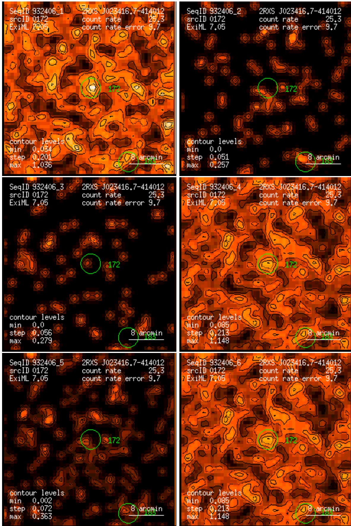
Figure 172: RASS 932406: detection 0172: band rate images, Gaussian filter: (1) PSPC channels 11 – 41, (2) 52 – 90, (3) 91 – 201, (4) 11 – 235, (5) 52 – 201, (6) 11 – 201. Broad band rates in counts/ks. Band rate contour levels in counts/ks/arcmin 2 .
