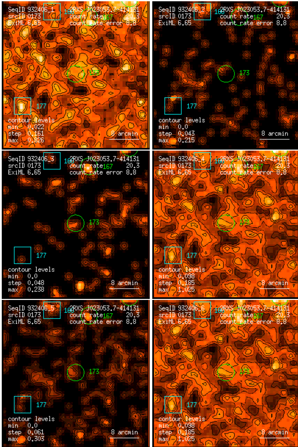
Figure 173: RASS 932406: detection 0173: band rate images, Gaussian filter: (1) PSPC channels 11 – 41, (2) 52 – 90, (3) 91 – 201, (4) 11 – 235, (5) 52 – 201, (6) 11 – 201. Broad band rates in counts/ks. Band rate contour levels in counts/ks/arcmin 2 .
