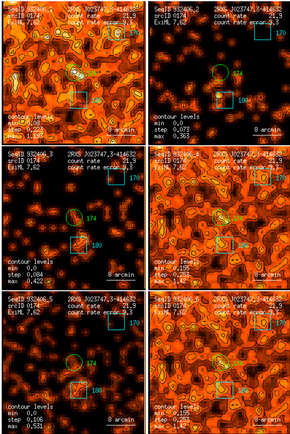
Figure 174: RASS 932406: detection 0174: band rate images, Gaussian filter: (1) PSPC channels 11 – 41, (2) 52 – 90, (3) 91 – 201, (4) 11 – 235, (5) 52 – 201, (6) 11 – 201. Broad band rates in counts/ks. Band rate contour levels in counts/ks/arcmin 2 .
