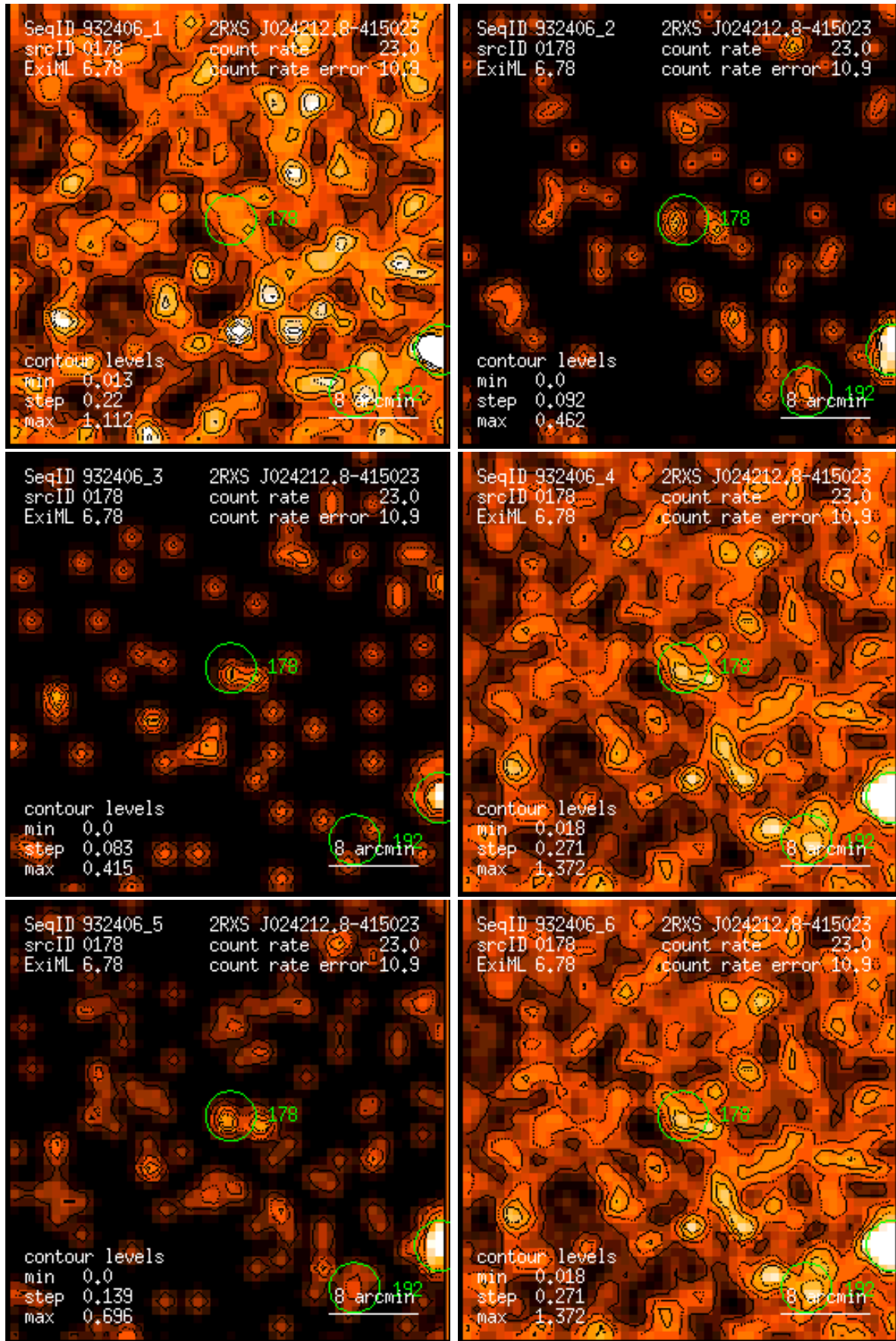
Figure 178: RASS 932406: detection 0178: band rate images, Gaussian filter: (1) PSPC channels 11 – 41, (2) 52 – 90, (3) 91 – 201, (4) 11 – 235, (5) 52 – 201, (6) 11 – 201. Broad band rates in counts/ks. Band rate contour levels in counts/ks/arcmin 2 .
