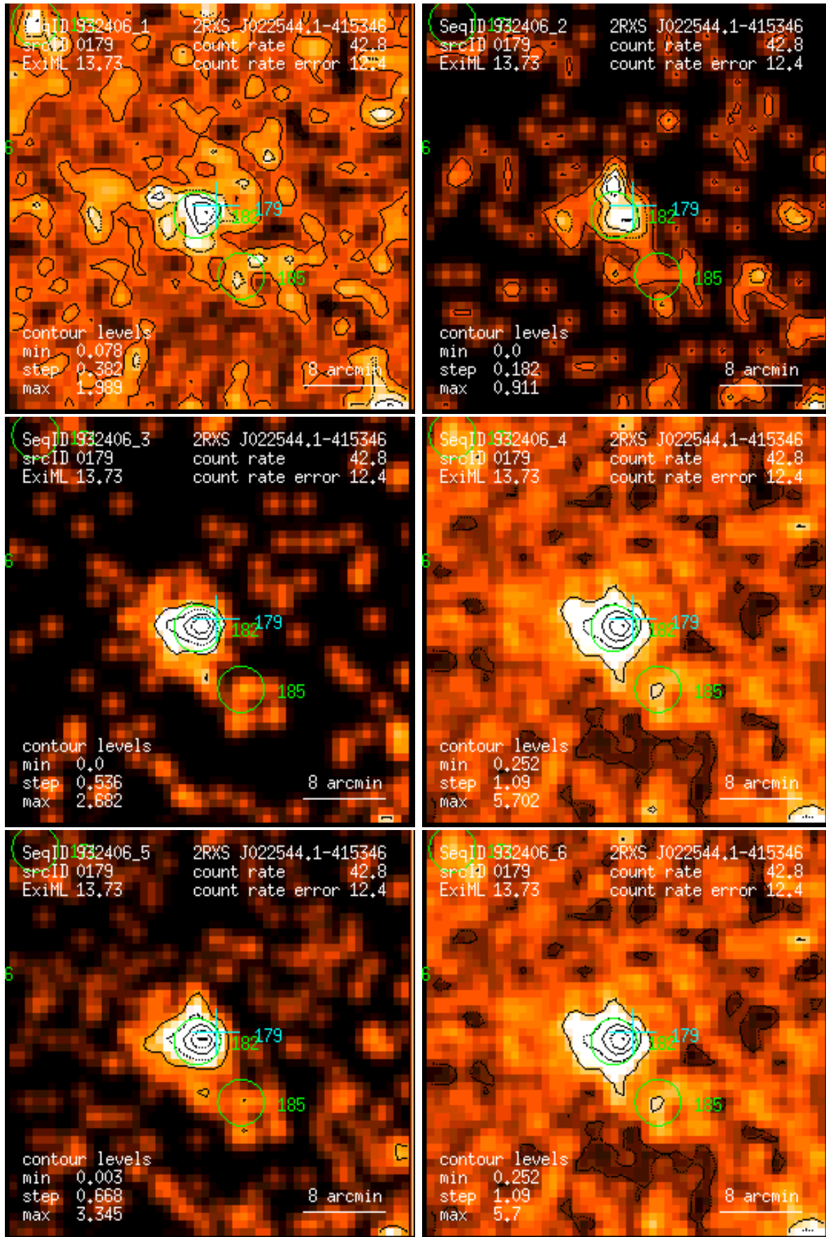
Figure 179: RASS 932406: detection 0179: band rate images, Gaussian filter: (1) PSPC channels 11 – 41, (2) 52 – 90, (3) 91 – 201, (4) 11 – 235, (5) 52 – 201, (6) 11 – 201. Broad band rates in counts/ks. Band rate contour levels in counts/ks/arcmin 2 .
