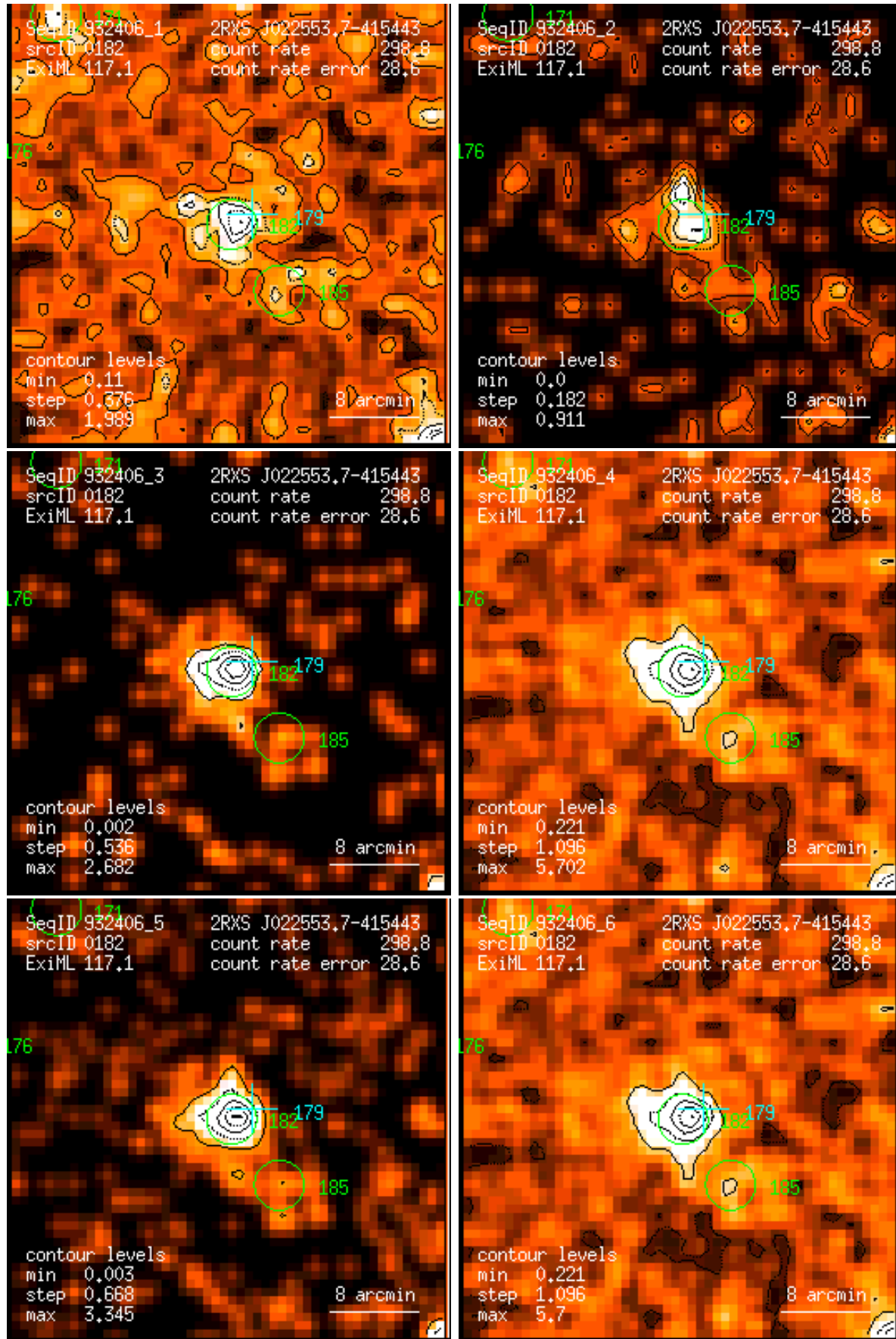
Figure 182: RASS 932406: detection 0182: band rate images, Gaussian filter: (1) PSPC channels 11 – 41, (2) 52 – 90, (3) 91 – 201, (4) 11 – 235, (5) 52 – 201, (6) 11 – 201. Broad band rates in counts/ks. Band rate contour levels in counts/ks/arcmin 2 .
