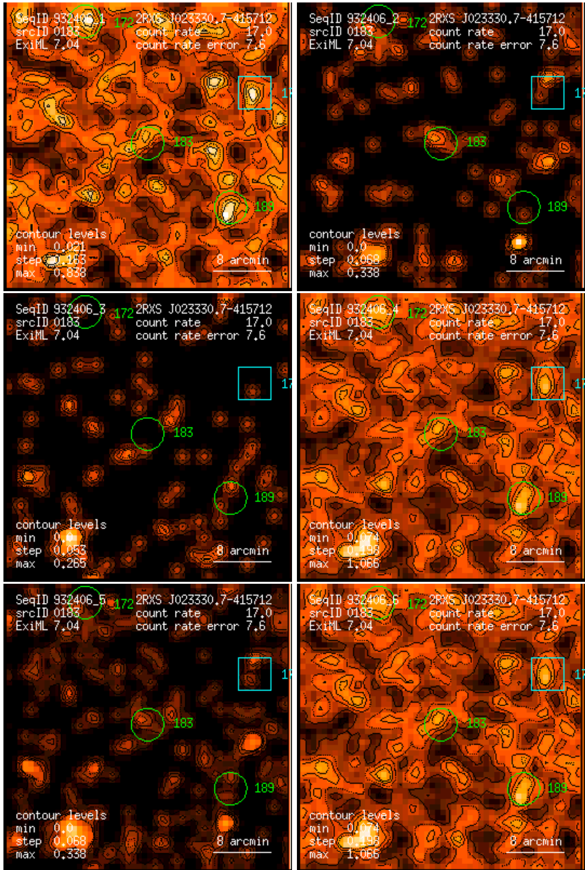
Figure 183: RASS 932406: detection 0183: band rate images, Gaussian filter: (1) PSPC channels 11 – 41, (2) 52 – 90, (3) 91 – 201, (4) 11 – 235, (5) 52 – 201, (6) 11 – 201. Broad band rates in counts/ks. Band rate contour levels in counts/ks/arcmin 2 .
