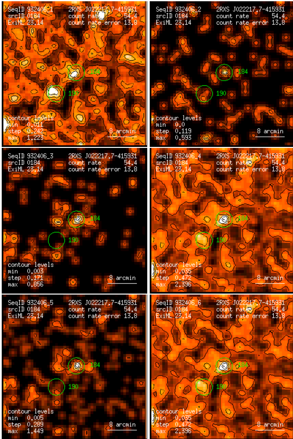
Figure 184: RASS 932406: detection 0184: band rate images, Gaussian filter: (1) PSPC channels 11 – 41, (2) 52 – 90, (3) 91 – 201, (4) 11 – 235, (5) 52 – 201, (6) 11 – 201. Broad band rates in counts/ks. Band rate contour levels in counts/ks/arcmin 2 .
