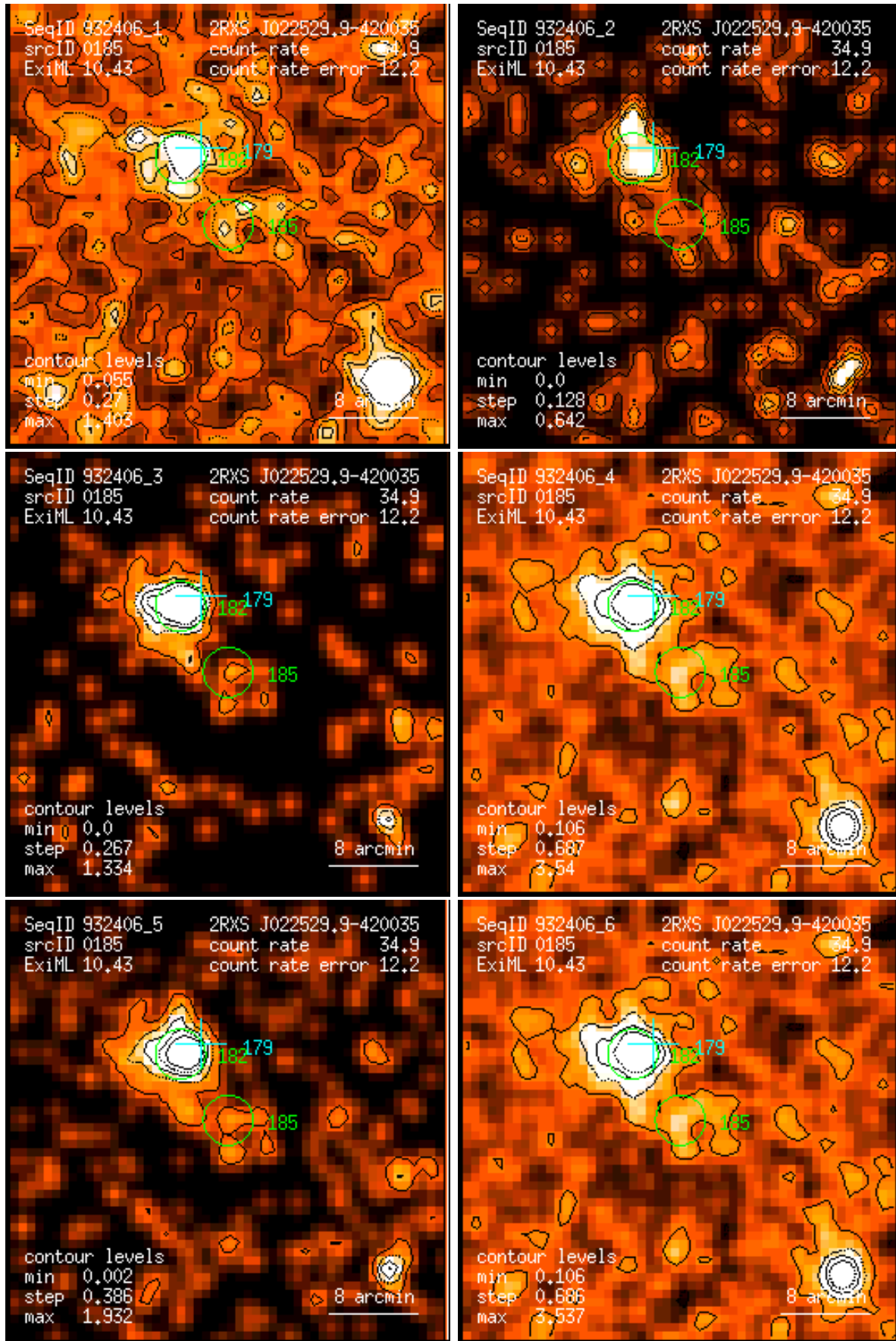
Figure 185: RASS 932406: detection 0185: band rate images, Gaussian filter: (1) PSPC channels 11 – 41, (2) 52 – 90, (3) 91 – 201, (4) 11 – 235, (5) 52 – 201, (6) 11 – 201. Broad band rates in counts/ks. Band rate contour levels in counts/ks/arcmin 2 .
