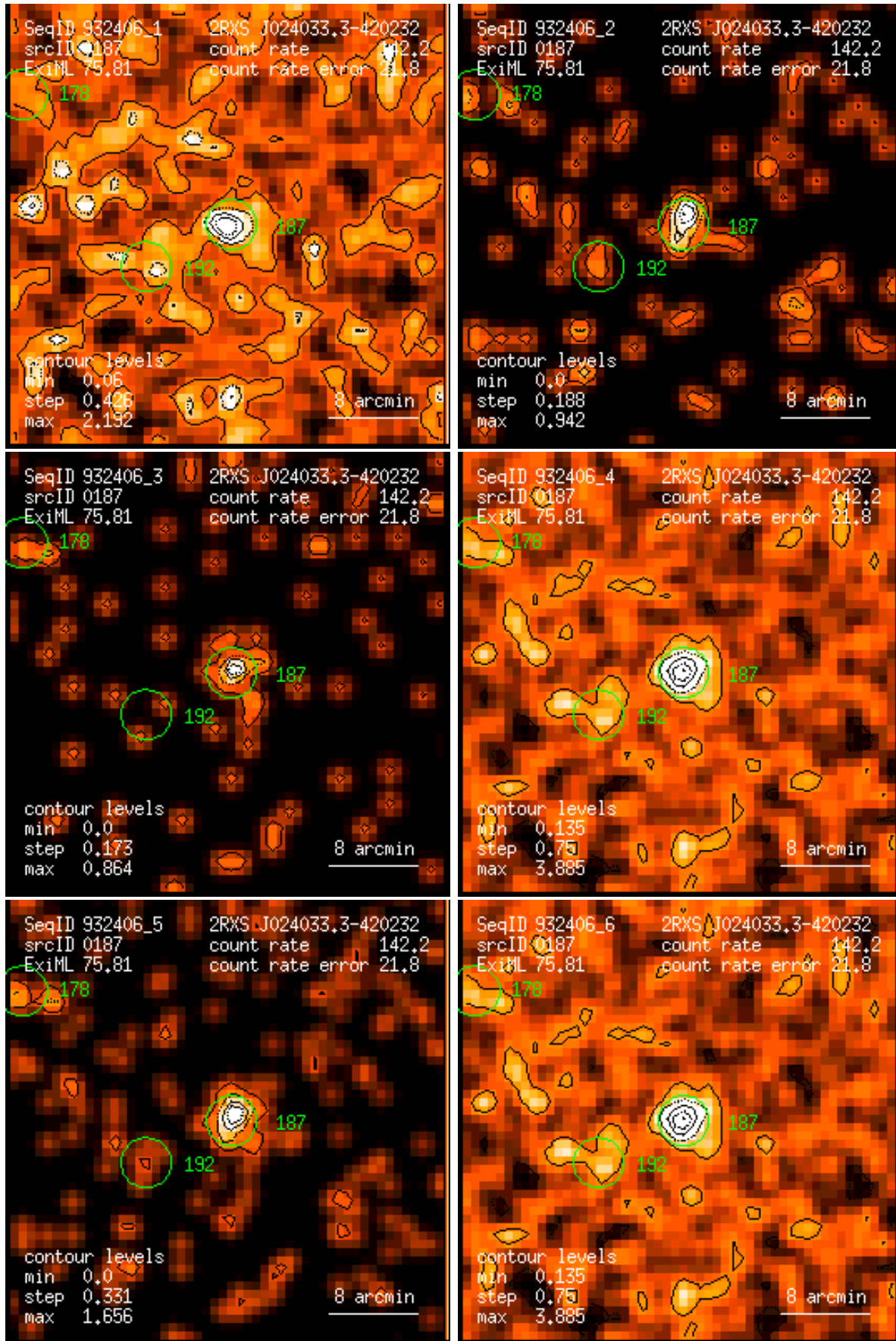
Figure 187: RASS 932406: detection 0187: band rate images, Gaussian filter: (1) PSPC channels 11 – 41, (2) 52 – 90, (3) 91 – 201, (4) 11 – 235, (5) 52 – 201, (6) 11 – 201. Broad band rates in counts/ks. Band rate contour levels in counts/ks/arcmin 2 .
