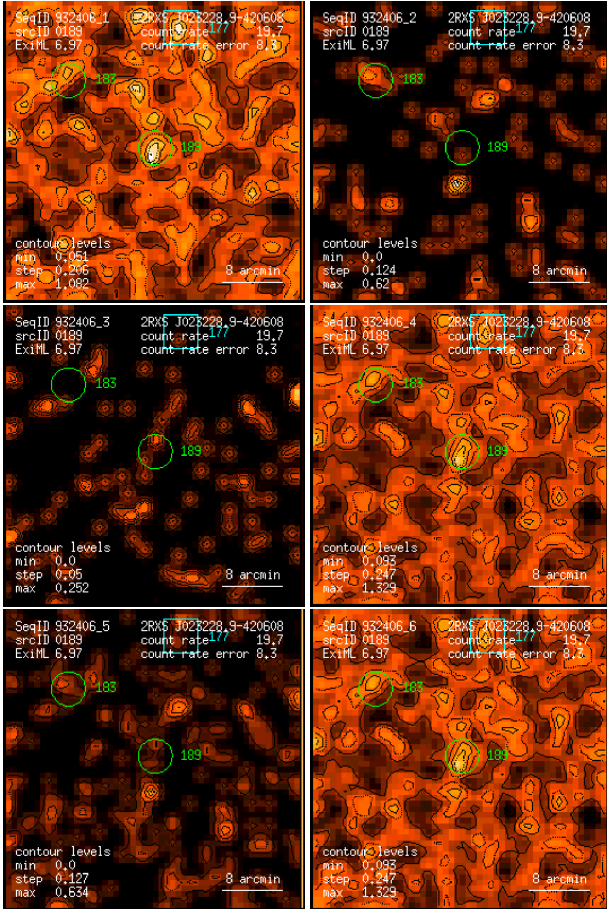
Figure 189: RASS 932406: detection 0189: band rate images, Gaussian filter: (1) PSPC channels 11 – 41, (2) 52 – 90, (3) 91 – 201, (4) 11 – 235, (5) 52 – 201, (6) 11 – 201. Broad band rates in counts/ks. Band rate contour levels in counts/ks/arcmin 2 .
