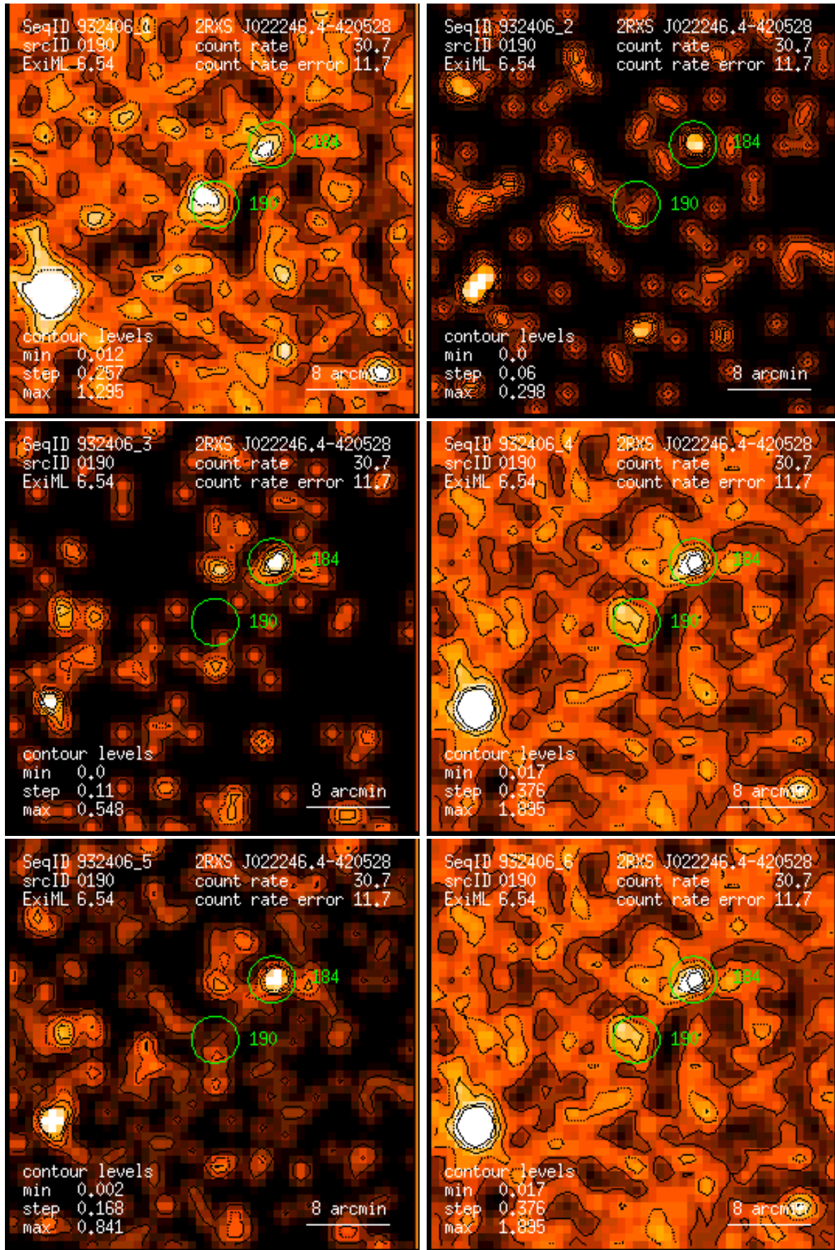
Figure 190: RASS 932406: detection 0190: band rate images, Gaussian filter: (1) PSPC channels 11 – 41, (2) 52 – 90, (3) 91 – 201, (4) 11 – 235, (5) 52 – 201, (6) 11 – 201. Broad band rates in counts/ks. Band rate contour levels in counts/ks/arcmin 2 .
