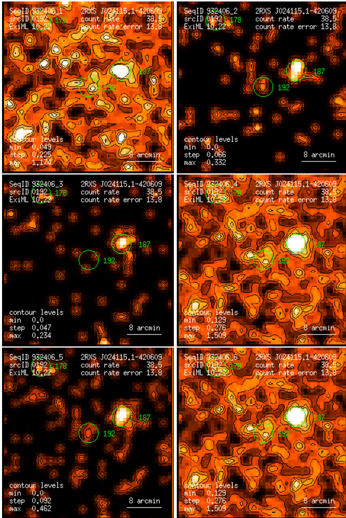
Figure 192: RASS 932406: detection 0192: band rate images, Gaussian filter: (1) PSPC channels 11 – 41, (2) 52 – 90, (3) 91 – 201, (4) 11 – 235, (5) 52 – 201, (6) 11 – 201. Broad band rates in counts/ks. Band rate contour levels in counts/ks/arcmin 2 .
