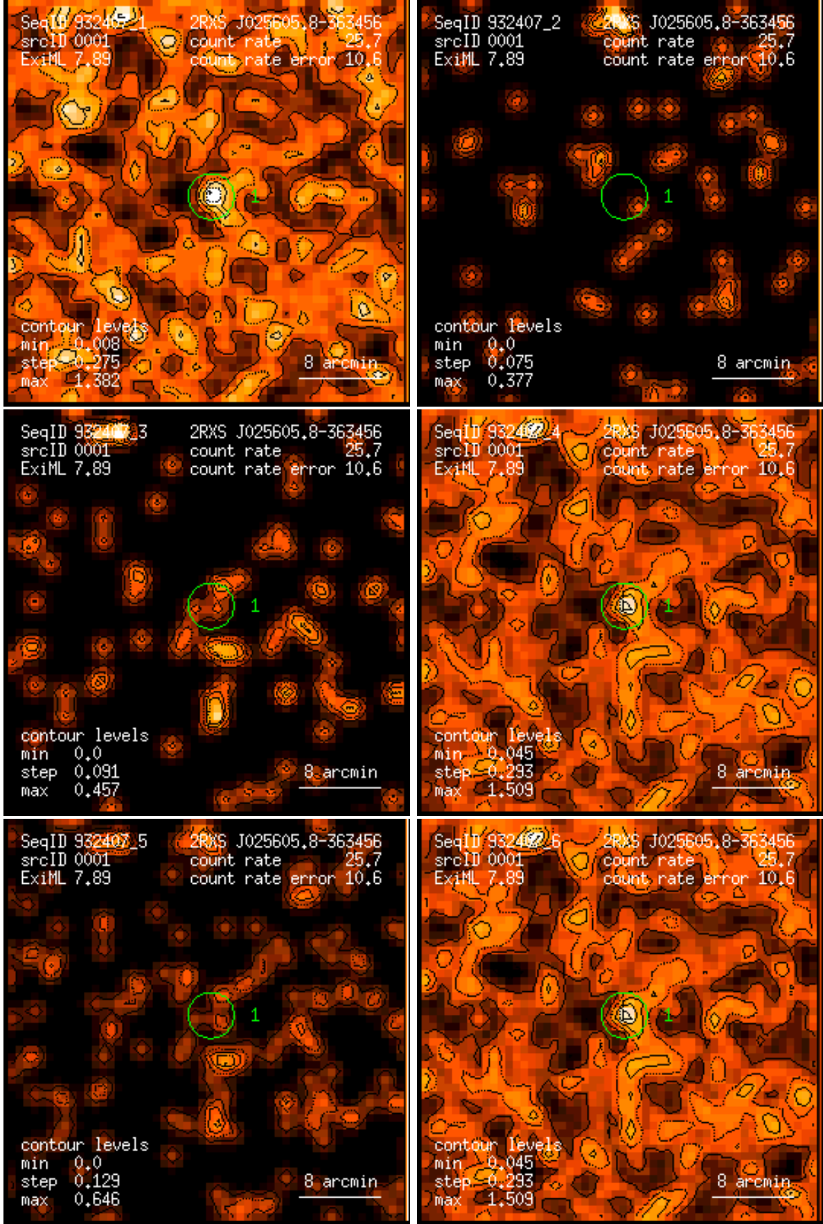
Figure 1: RASS 932407: detection 0001: band rate images, Gaussian filter: (1) PSPC channels 11 – 41, (2) 52 – 90, (3) 91 – 201, (4) 11 – 235, (5) 52 – 201, (6) 11 – 201. Broad band rates in counts/ks. Band rate contour levels in counts/ks/arcmin 2 .
