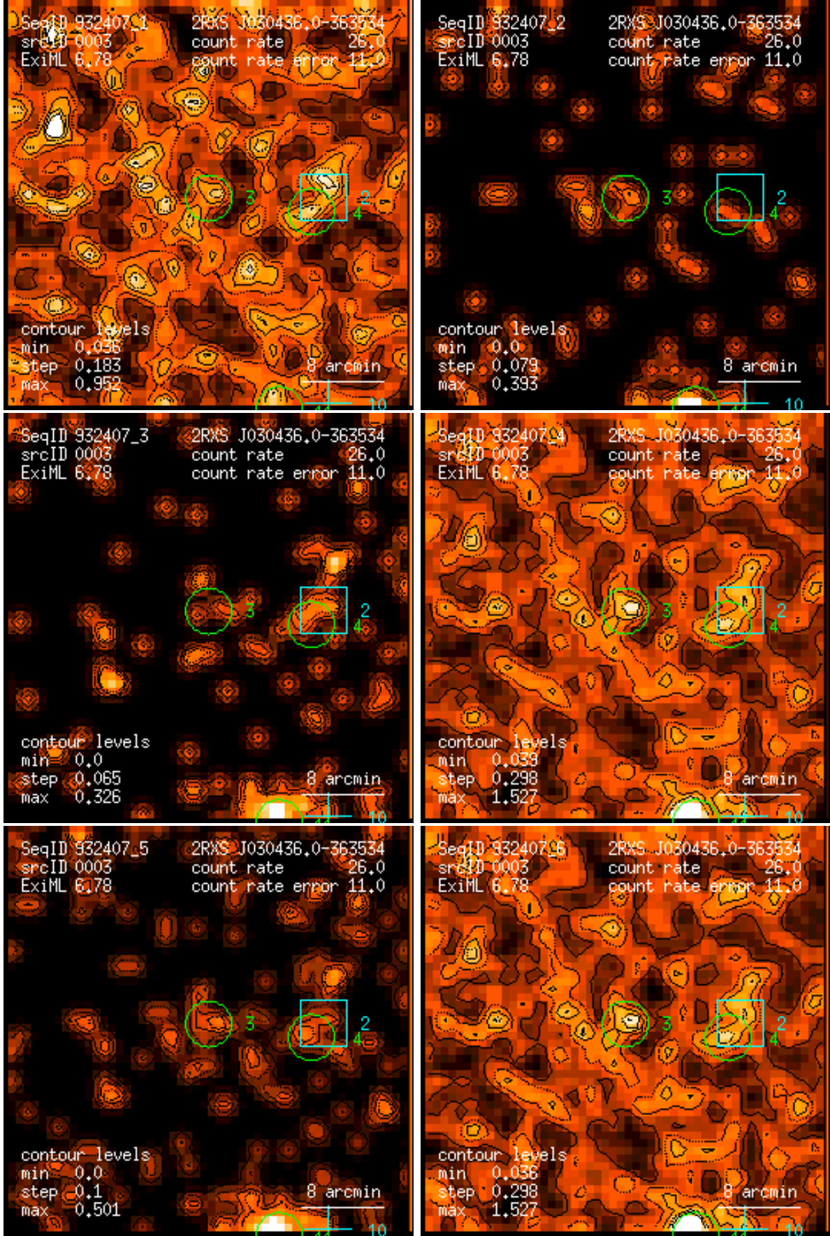
Figure 3: RASS 932407: detection 0003: band rate images, Gaussian filter: (1) PSPC channels 11 – 41, (2) 52 – 90, (3) 91 – 201, (4) 11 – 235, (5) 52 – 201, (6) 11 – 201. Broad band rates in counts/ks. Band rate contour levels in counts/ks/arcmin 2 .
