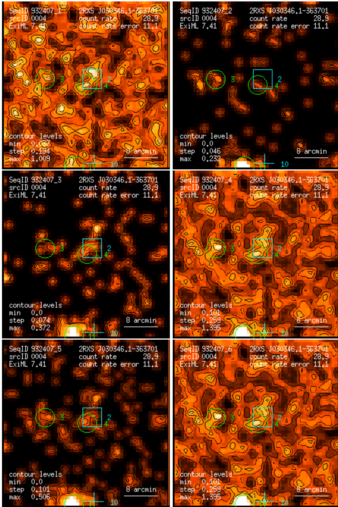
Figure 4: RASS 932407: detection 0004: band rate images, Gaussian filter: (1) PSPC channels 11 – 41, (2) 52 – 90, (3) 91 – 201, (4) 11 – 235, (5) 52 – 201, (6) 11 – 201. Broad band rates in counts/ks. Band rate contour levels in counts/ks/arcmin 2 .
