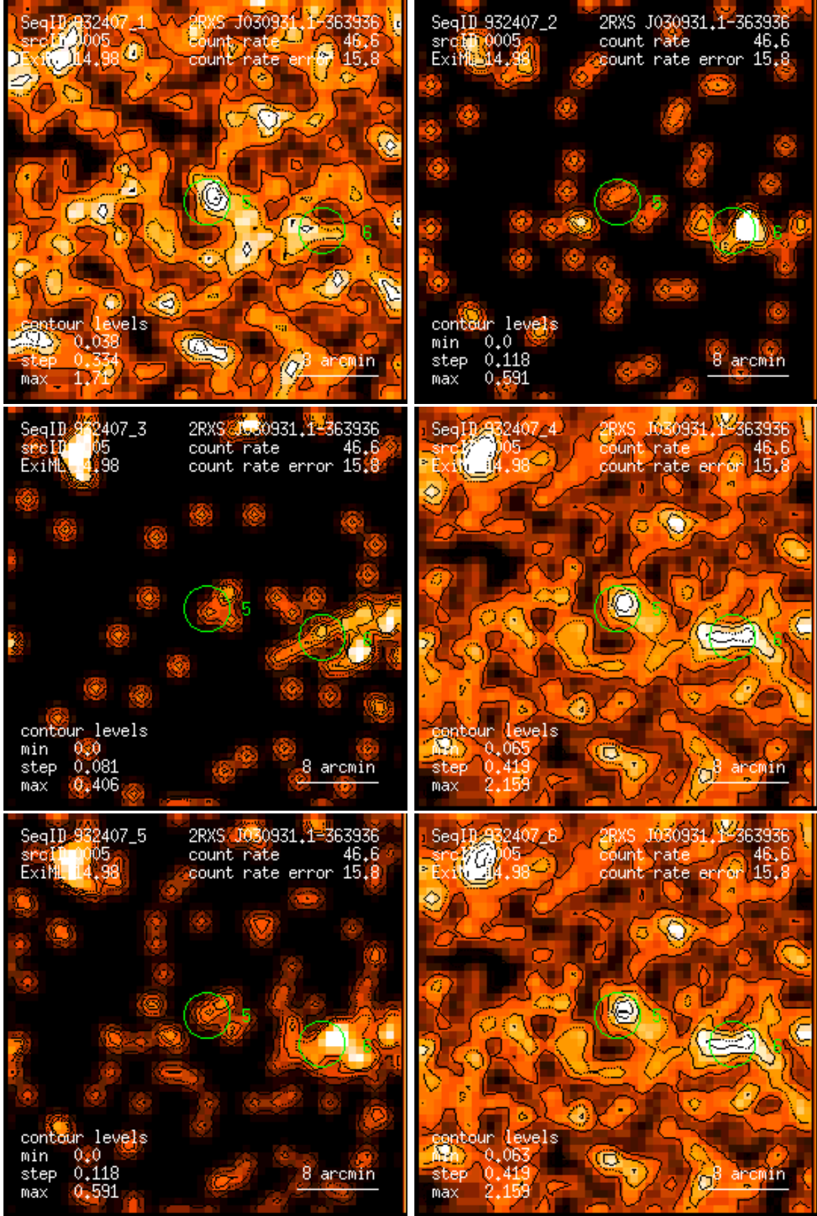
Figure 5: RASS 932407: detection 0005: band rate images, Gaussian filter: (1) PSPC channels 11 – 41, (2) 52 – 90, (3) 91 – 201, (4) 11 – 235, (5) 52 – 201, (6) 11 – 201. Broad band rates in counts/ks. Band rate contour levels in counts/ks/arcmin 2 .
