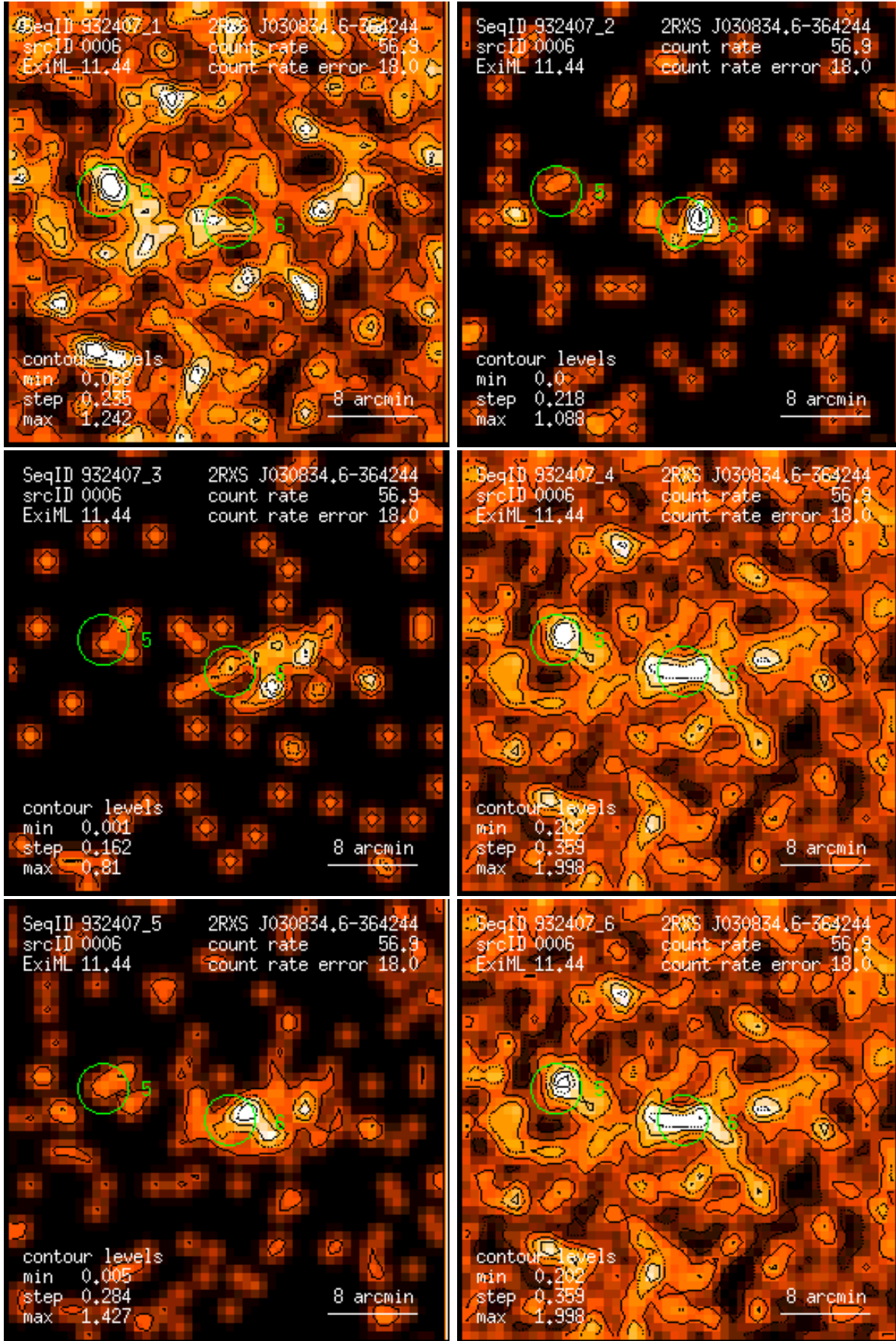
Figure 6: RASS 932407: detection 0006: band rate images, Gaussian filter: (1) PSPC channels 11 – 41, (2) 52 – 90, (3) 91 – 201, (4) 11 – 235, (5) 52 – 201, (6) 11 – 201. Broad band rates in counts/ks. Band rate contour levels in counts/ks/arcmin 2 .
