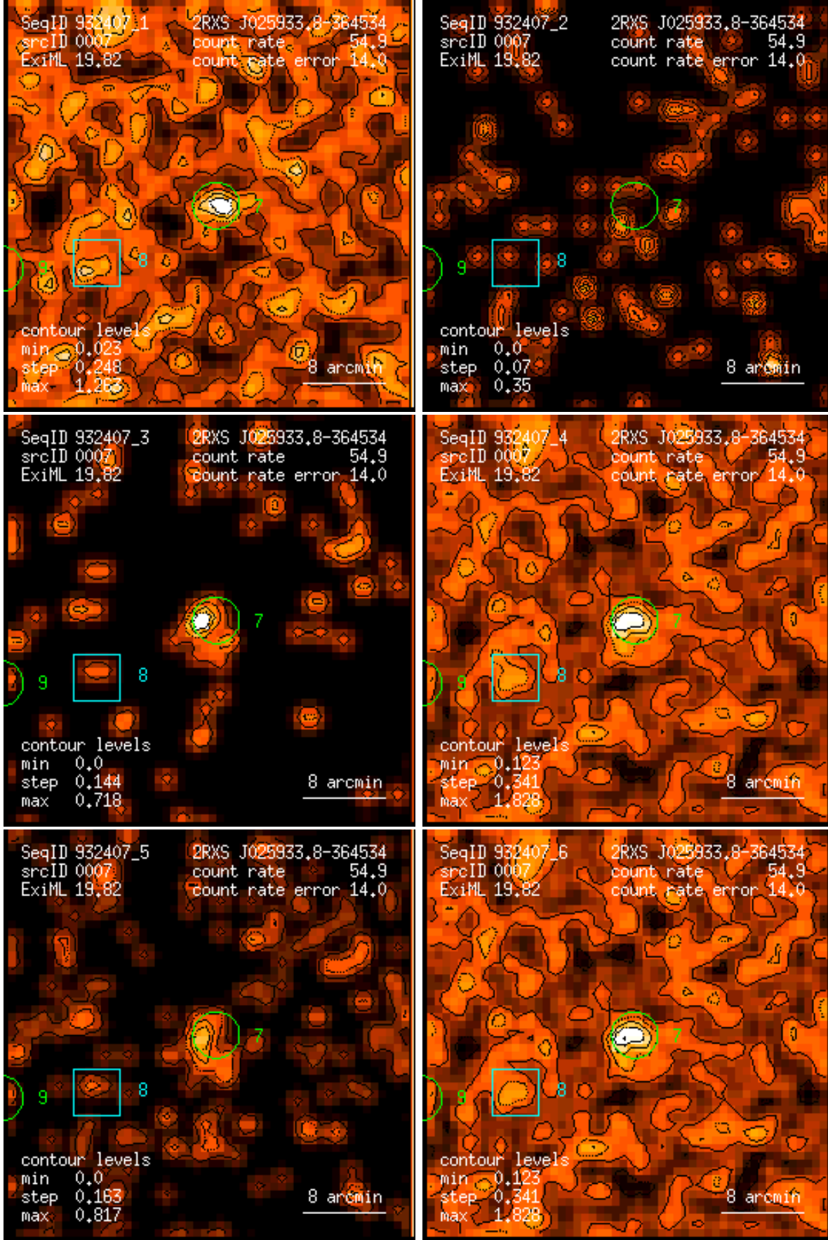
Figure 7: RASS 932407: detection 0007: band rate images, Gaussian filter: (1) PSPC channels 11 – 41, (2) 52 – 90, (3) 91 – 201, (4) 11 – 235, (5) 52 – 201, (6) 11 – 201. Broad band rates in counts/ks. Band rate contour levels in counts/ks/arcmin 2 .
