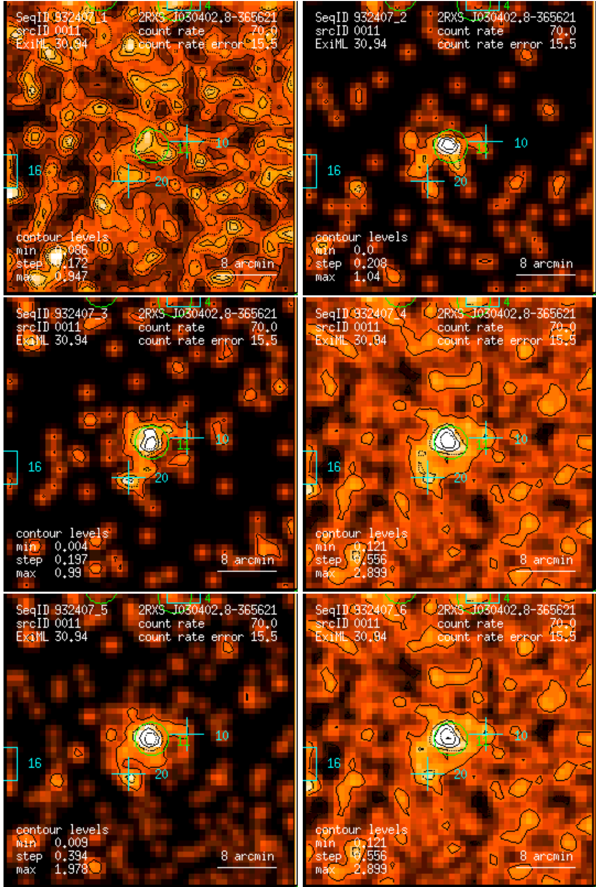
Figure 11: RASS 932407: detection 0011: band rate images, Gaussian filter: (1) PSPC channels 11 – 41, (2) 52 – 90, (3) 91 – 201, (4) 11 – 235, (5) 52 – 201, (6) 11 – 201. Broad band rates in counts/ks. Band rate contour levels in counts/ks/arcmin 2 .
