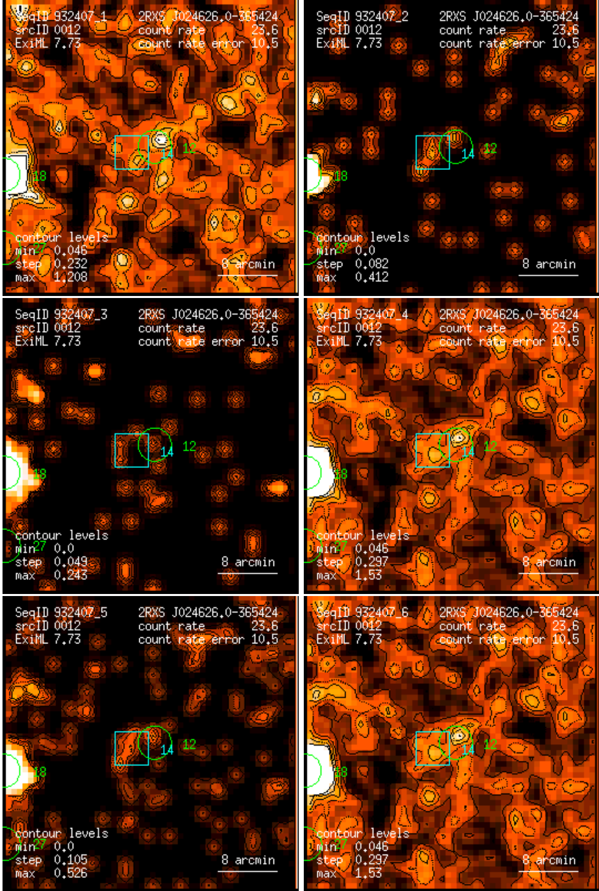
Figure 12: RASS 932407: detection 0012: band rate images, Gaussian filter: (1) PSPC channels 11 – 41, (2) 52 – 90, (3) 91 – 201, (4) 11 – 235, (5) 52 – 201, (6) 11 – 201. Broad band rates in counts/ks. Band rate contour levels in counts/ks/arcmin 2 .
