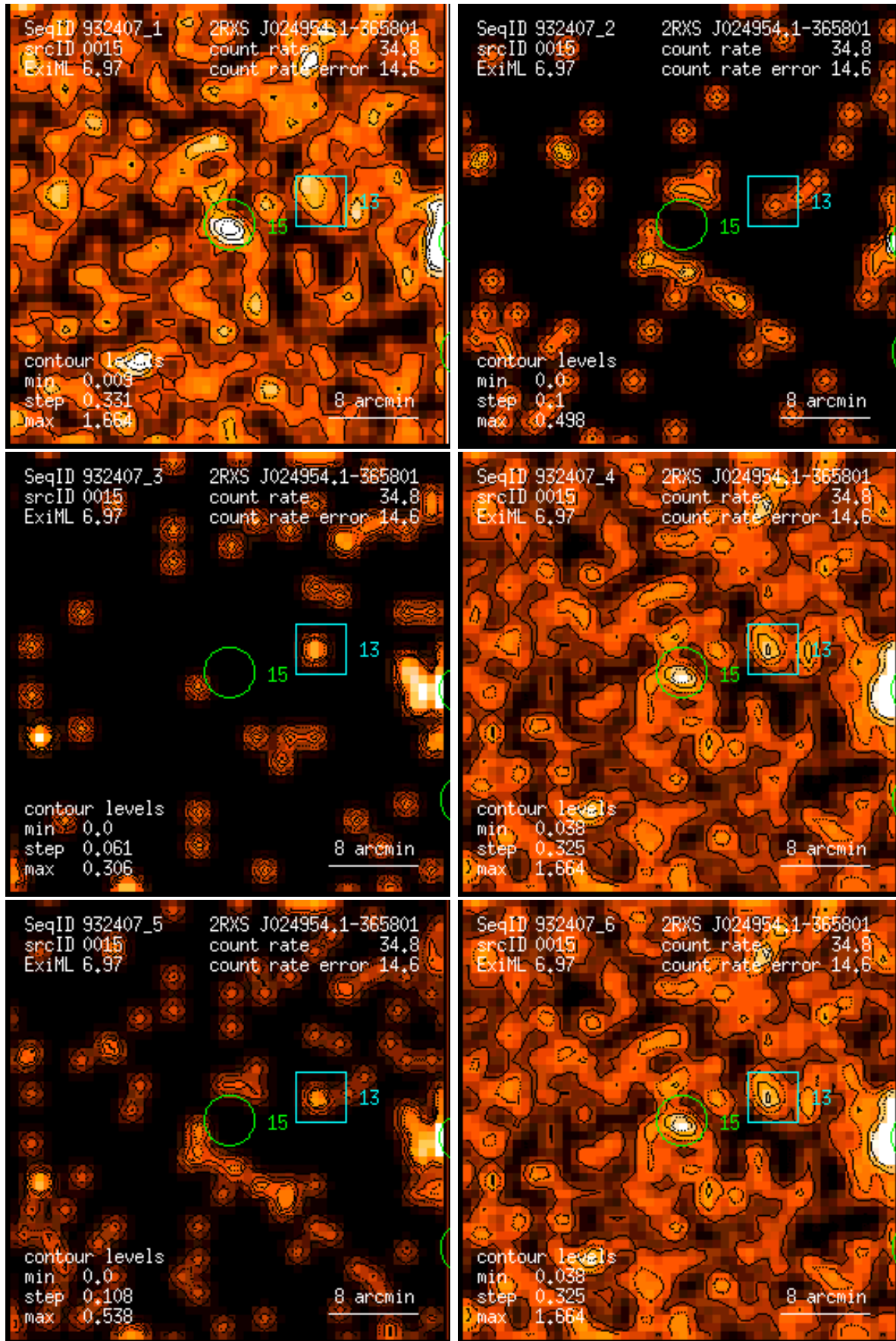
Figure 15: RASS 932407: detection 0015: band rate images, Gaussian filter: (1) PSPC channels 11 – 41, (2) 52 – 90, (3) 91 – 201, (4) 11 – 235, (5) 52 – 201, (6) 11 – 201. Broad band rates in counts/ks. Band rate contour levels in counts/ks/arcmin 2 .
