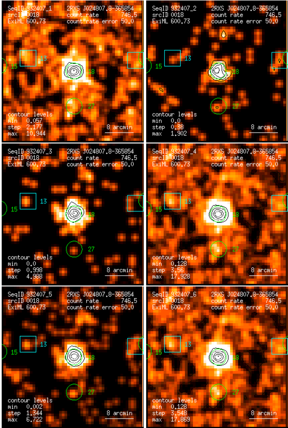
Figure 18: RASS 932407: detection 0018: band rate images, Gaussian filter: (1) PSPC channels 11 – 41, (2) 52 – 90, (3) 91 – 201, (4) 11 – 235, (5) 52 – 201, (6) 11 – 201. Broad band rates in counts/ks. Band rate contour levels in counts/ks/arcmin 2 .
