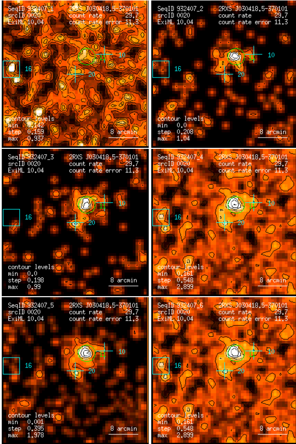
Figure 20: RASS 932407: detection 0020: band rate images, Gaussian filter: (1) PSPC channels 11 – 41, (2) 52 – 90, (3) 91 – 201, (4) 11 – 235, (5) 52 – 201, (6) 11 – 201. Broad band rates in counts/ks. Band rate contour levels in counts/ks/arcmin 2 .
